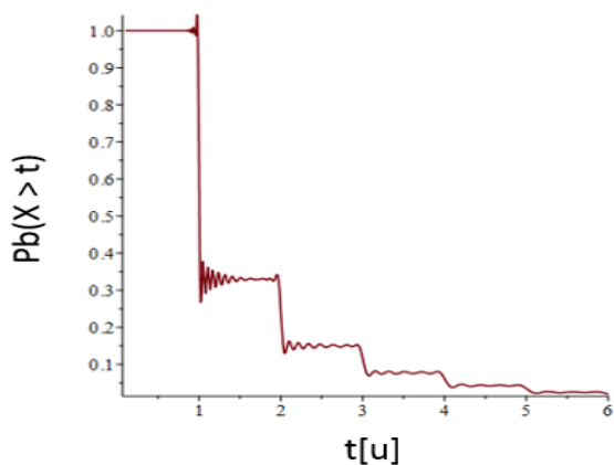
Figure 3. Distribution of the busy period Pb(X > t) for \lambda = 0.4 , t is in time unit (u).
