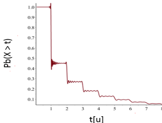
Figure 5. Distribution of the busy period Pb(X > t) for \lambda = 0.8 , t is in time unit (u).
