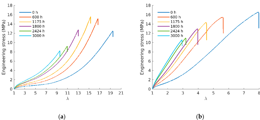
Figure 2. (a) Tensile curves to failure of samples aged at 90 °C for unfilled and (b) filled rubbers.
