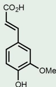
Ferulic acid
