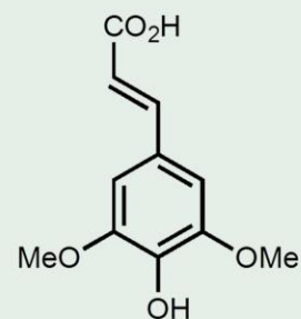
Sinapic acid
