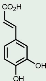
Caffeic acid
