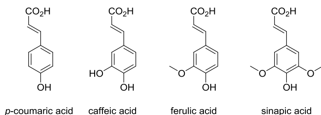
Figure 1. Structures of the main naturally occurring p -hydroxycinnamic acids.
