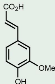
Ferulic acid
