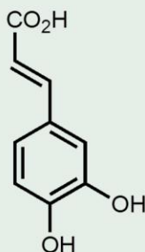
Caffeic acid
