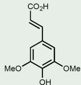
Sinapic acid
