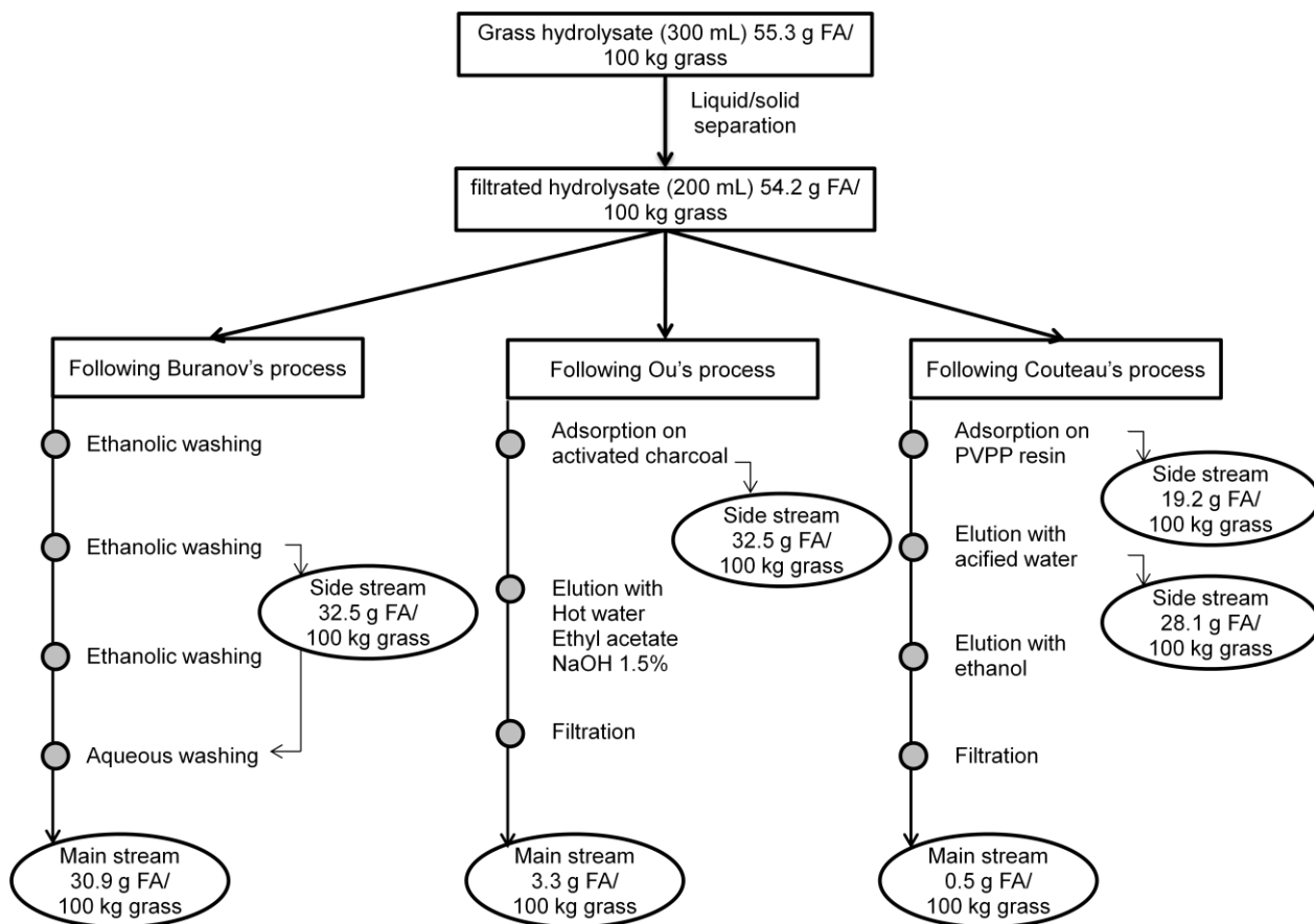
Scheme 2. Simplified flow chart of processes followed by Salgado et al. [102]
