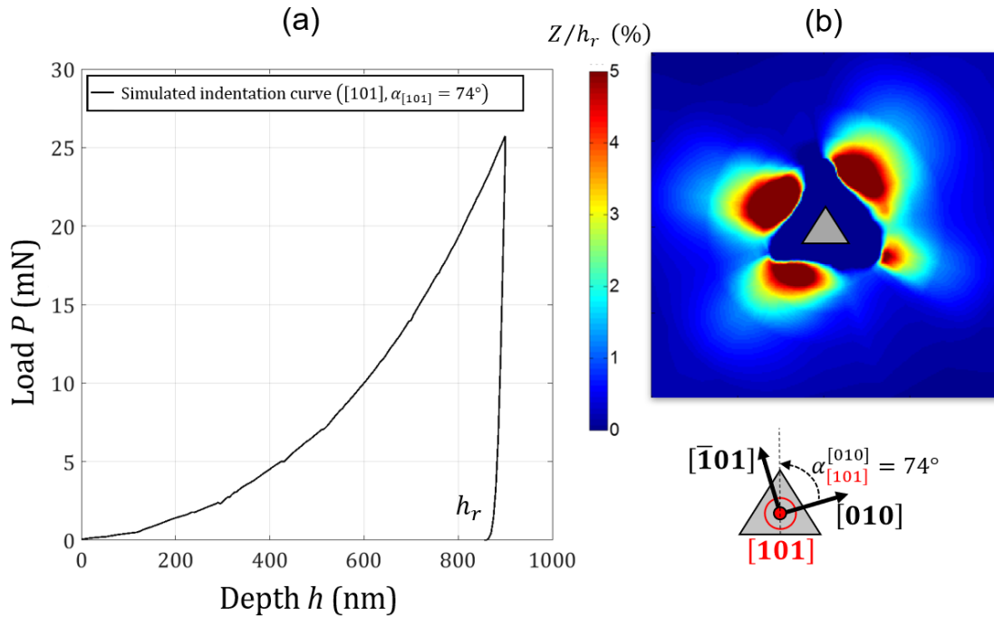
Figure 3 - Nanoindentation CPFEM simulation performed in the [101] grain orientation with azimuth \alpha_{[101]}^{[010]} = 74^\circ using the virtual material: (a) indentation curve \mathbf{P} , (b) residual topography
