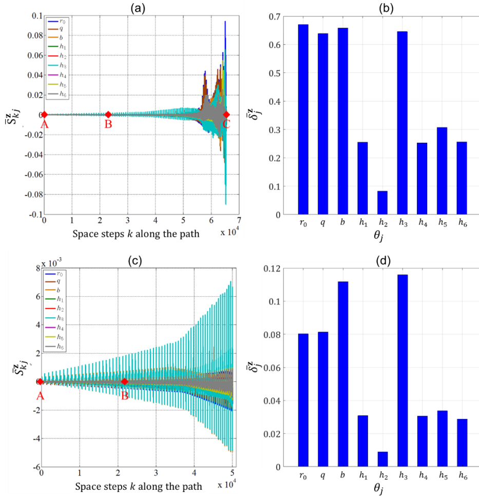
Figure 8 - Entire imprint topography \mathbf{Z} = \mathbf{Z}^1 : (a) sensitivity vectors \bar{S}_{kj}^z and (b) norms \bar{\delta}_j^z = \sqrt{\bar{S}_{kj}^z \bar{S}_{kj}^z} . Truncated imprint: (c) sensitivity vectors and (d) norms.
