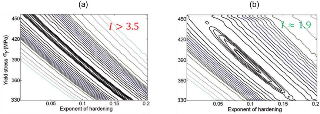
Figure 10 – Objective functions iso-values obtained by Bolzon et al. using macroscopic FEM (Bolzon et al., 2011): (a) indentation curve only I > 3.5 , (b) residual profile only I \approx 1.9 . I -index values graphically estimated.
