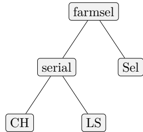
Figure 2: GRASP skeleton tree
