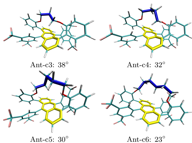
Figure 8. Structures of Ant- cn , where n = 3 - 6 . From left to right and top to bottom: Ant-c3 (torsion angle 38°), Ant-c4 (torsion angle 32°), Ant-c5 (torsion angle 30°), Ant-c6 (torsion angle 23°). The torsion angle is defined as the angle between the ends of the central anthracene. In each case, the anthracene itself is highlighted in yellow, while the carbon bridge that determines the torsion is highlighted in blue.
