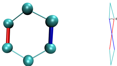
Figure 7. Dihedral torsion of a benzene ring, viewed from the front (left) and the side (right). In this work, the dihedral torsion of an individual benzene ring is defined as the maximum angle \theta between any two opposing bonds in the ring.
