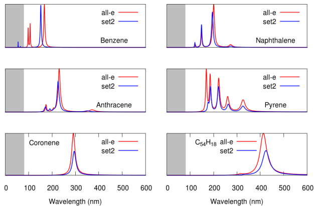
Figure 1. Comparison of the absorption spectra for the 20 first singlet excitations obtained with set2 pseudopotentials and all-electron calculations (def2-SV(P)(s-less)/TD-PBE0) within the RPA framework. The grey zone covers energies for which no all-electron excitations have been calculated.
