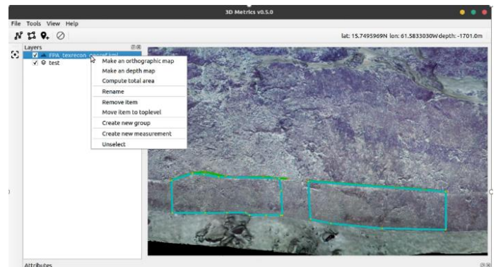
Figure 4: Example of measurement in 3DMetrics on a geologic fault.
