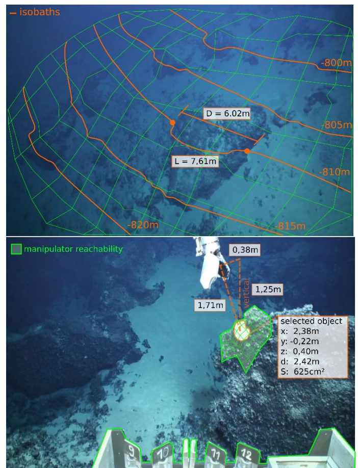
Figure 3: In-dive augmented perception for operator assistance in direct interaction with the environment.
