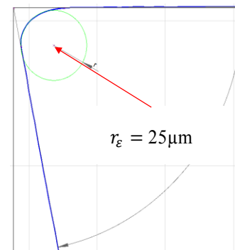
Fig. 1. Measurement of the edge radius
