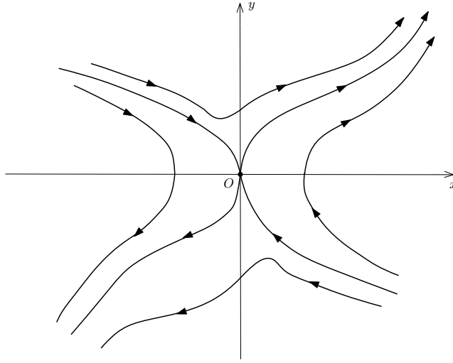
FIGURE 1. Phase portrait of X_c^E for \alpha < 1 . It fulfills some differentiable features of the flow such as the contact of orbits at the origin.
