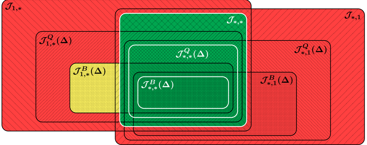
Figure 1: Stabilizing leader election: summary of the results. Pseudo- (and so self-) stabilizing leader election is impossible in the red area. Self- (and so pseudo-) stabilizing leader election is possible in the green area. In the yellow area, only pseudo-stabilization can be achieved.
