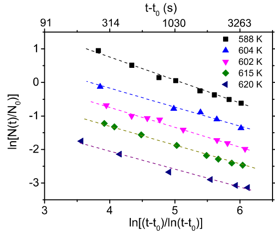
Figure 4: Ln of the normalized evolution of the number of droplets as function of \ln[(t-t_0)/\ln(t-t_0)] for different temperatures. For clarity the data are offset vertically. The dashed lines show the asymptotic fit of the data.
