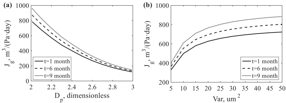
Fig. 6. (a) Relationship between gas injectivity index and fractal dimension at different time and (b) relationship between gas injectivity index and variance at different time.
