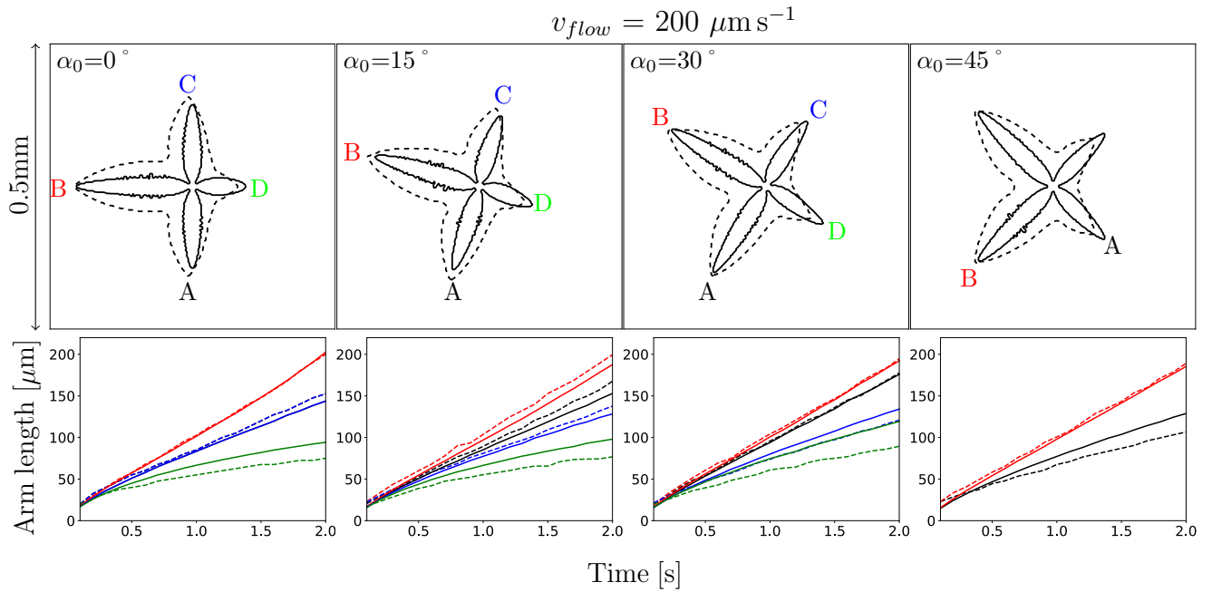
Fig. 4: Equiaxed dendrite growth in forced flow at v_{flow} = 200 \mu\text{m/s} \approx 6V_{diff} for different orientations \alpha_0 with respect to the flow. Top : Solid-liquid interface for the phase-field model (solid line) and dendrite envelope for the mesoscopic model (dashed line) at t = 2 \text{ s} . Bottom: Evolution of the lengths of the four primary arms. Phase field is shown in solid line and the mesoscopic model in dashed line. Note that for \alpha_0 = 0^\circ the lengths of arms A and C are identical and that for \alpha_0 = 45^\circ the two upstream arms (B) and the two downstream arms (A) are identical.
