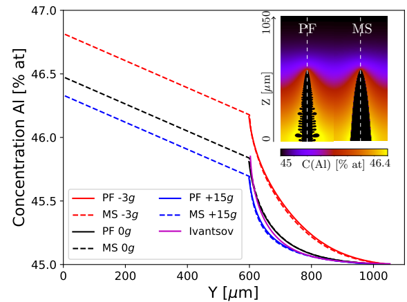
Fig. 12: Concentration profiles in the liquid in front of the primary tip at gravity levels between -3g and +15g for phase field (PF) and for the mesoscopic model (MS) at 200s . The inset shows the position of the profiles. The analytical solution of the concentration profile in front of a free tip (Ivantsov) growing at the same speed is shown for comparison.
