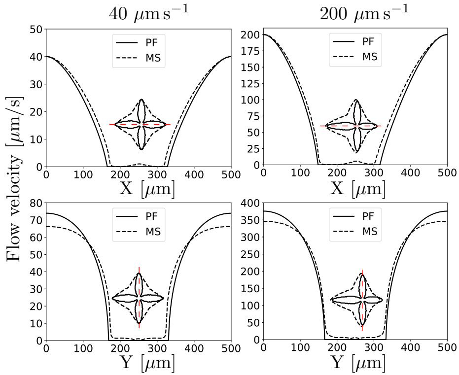
Supplementary Fig. 3. Velocity magnitude profiles for different forced flow velocities ( 40 and 200 \mu\text{m/s} ) along the X -axis (top) and the Y -axis (bottom) at t = 1 s for the mesoscopic model (MS) and for phase field (PF). The insets show the positions of the profiles.
