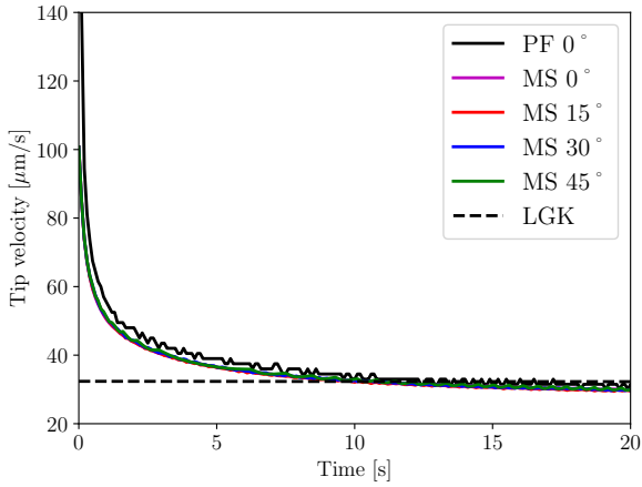
Fig. 2: Evolution of the primary tip velocity in diffusive growth: results of the mesoscopic model (MS) for orientations of \alpha_0 = 0^\circ , 15^\circ , 30^\circ and 45^\circ with respect to the grid are compared to the phase-field model (PF) for \alpha_0 = 0^\circ . The dashed line shows the LGK analytical solution [59] for the steady state.
