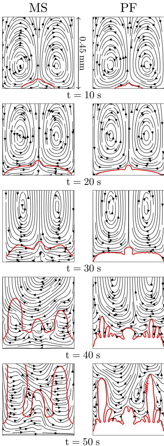
Fig. 11: Early stage branch competition under the influence of buoyancy-driven convection at a gravity level of -10g for the mesoscopic model (MS) and for phase field (PF). Streamlines, dendrite envelope (MS), and solid-liquid interface (PF).
