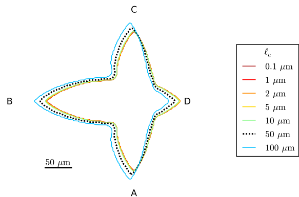
Fig. 6: Influence of the characteristic length, \ell_c , used for the permeability on the shape of the dendrite envelope predicted by the mesoscopic model. Note that the permeability K \sim (\ell_c)^2 . The comparison is made for v_{\text{flow}} = 200 \mu\text{m/s} at t = 1.8 s. The stagnant-film thickness is \delta = 0.20 l_{\text{diff}} in all cases.
