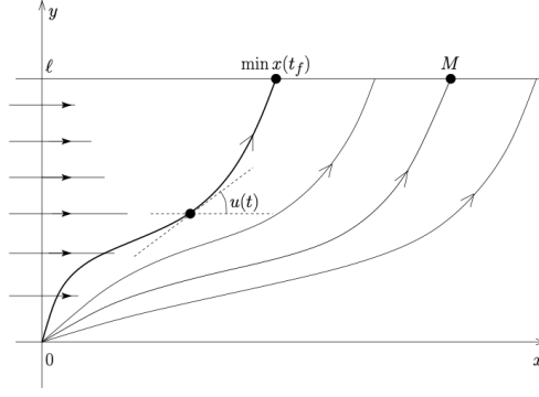
Figure 1: Zermelo problem.
