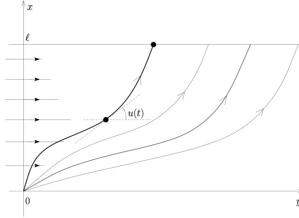
Figure 1: Zermelo problem.
