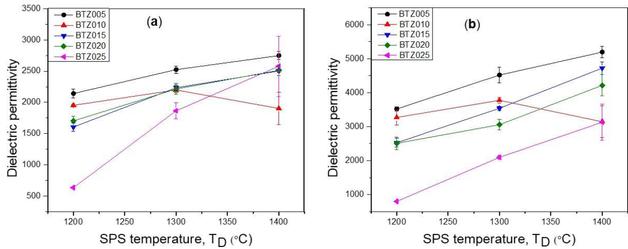
Figure 7: Dielectric permittivity at (a) room (25 ^{\circ}C ) and (b) Curie ( T_c ) temperature of BaTi_{(1-x)}Zr_xO_3 ( x=0.05-0.25 ) ceramics as a function of T_D .
