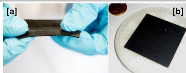
Figure 10. [a] Composite containing 5% wt. of TTF-TCNQ nanoparticles in a space-qualified resin, thickness: 0.4 mm. ©Frédéric MALIGNÉ/LCC/CNRS Photothèque, Copyright (2018), with permission from CNRS Photothèque. [b] Alumina substrate (5 cm × 5 cm) covered by a continuous deposit of TTF-TCNQ nanoparticles, thickness = 90.00 ± 0.04 μm. Reproduced from ref. [14f] , Copyright (2013), with permission from the American Chemical Society.
