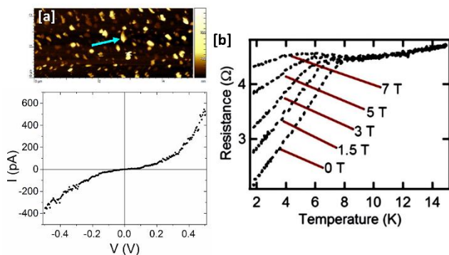
Figure 9. [a] AFM topographic image of Per 2 [Au(mnt) 2 ] and I-V curve of a 40 nm high nanoparticle indicated by the arrow. Reproduced from ref. [16] , Copyright (2020), with permission from the Académie des Sciences, Paris; [b] Temperature dependent resistance of Et 2 I 3 nanoparticles at various magnetic fields up to 7 T confirming a superconducting transition for all applied fields. Reproduced from ref. [19] , Copyright (2016), with permission from the Royal Society of Chemistry.
