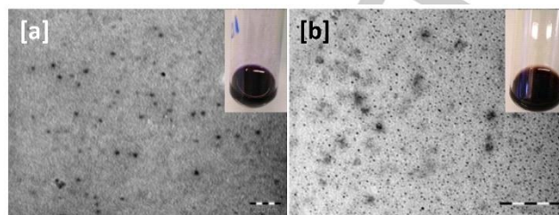
Figure 12. TEM images of [a] TTF-TCNQ/ n -Oct and [b] TTF-TCNQ/ n -Oct/ trans -2-decenoic acid nanoparticles from the 2.5 \text{g}\cdot\text{L}^{-1} solutions in ethanol (inserts): scale bars = 200 nm. Adapted from ref. [14h] , Copyright (2020), with permission from The Royal Society of Chemistry.
