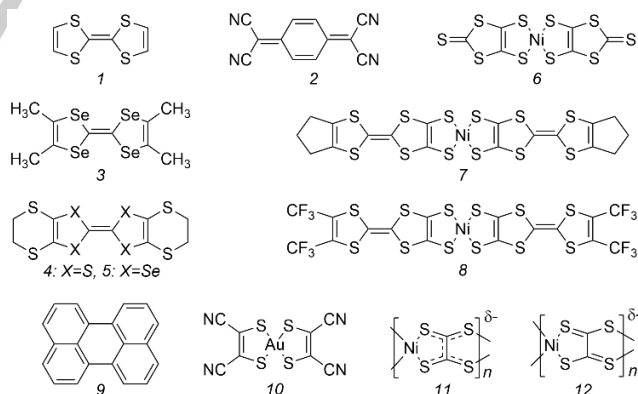
Figure 1. Molecular structures of cited building blocks of molecular conductors. 1) tetrathiafulvalene or TTF; 2) tetracyanoquinodimethane or TCNQ; 3) tetramethyltetraselenafulvalene or TMTSF; 4) bis(ethylenedithio)tetrathiafulvalene or BEDT-TTF or ET; 5) bis(ethylenedithio)tetraselenafulvalene or BETS; 6) nickel-bis(1,3-dithiol-2-thione-4,5-dithiolate) or nickel-dimercaptoisotrithione or Ni(dmit) 2 ; 7) nickel-bis(trimethylenetetrafulvalenedithiolate) or Ni(tmdt) 2 ; 8) nickel-bis(trifluoromethyltetrathiafulvalenedithiolate) or Ni(hfdt) 2 ; 9) perylene or Per; 10) gold-bis(dicyano-1,2-ethylenedithiolate) or gold-bis(maleonitriledithiolate) or Au(mnt) 2 ; 11) nickel-ethylenetetrafulvalene or Ni(ett); 12) nickel-tetrafulvalene or Ni(tto).
