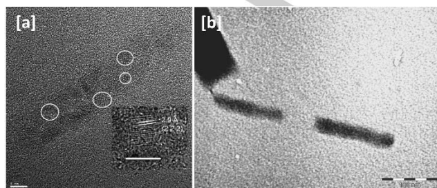
Figure 8. [a] HRTEM image of 3–5 nm aggregated crystalline nanoparticles of (TMTSF) 2 ClO 4 /[Me( n -Oct) 3 N]ClO 4 . Inset: one indexed 4.5 nm nanoparticle, (scale bar = 5 nm). Reproduced from ref. [15b] ; [b] High magnification TEM image of TTFBr 0.56 /PEDOT nanosticks resulting from a super-organization of particles (scale bar = 100 nm). Reproduced from ref. [18] , Copyright (2011), with permission from Elsevier.
