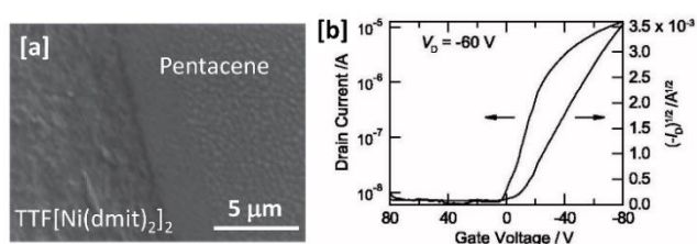
Figure 11. [a] SEM image of a boundary of TTF[Ni(dmit) 2 ] 2 electrode and pentacene channel regions. Reproduced from ref. [14c] , Copyright (2011), with permission from the Royal Society of Chemistry. [b] Transfer characteristics of pentacene OFETs with source/drain electrodes made from TTF-TCNQ nanoparticles. Reproduced from ref. [14b] , Copyright (2011), with permission from the Royal Society of Chemistry (RSC) on behalf of the Centre National de la Recherche Scientifique (CNRS) and the RSC.
