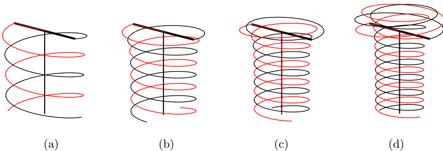
FIGURE 5. Vortex geometry for a two bladed rotor in helicopter regimes. (a) \lambda = -10 , (b) \lambda = \infty , (c) \lambda = 19 , (d) \lambda = 11 . For all cases \eta = 0.05 and \varepsilon = 0.01 .
