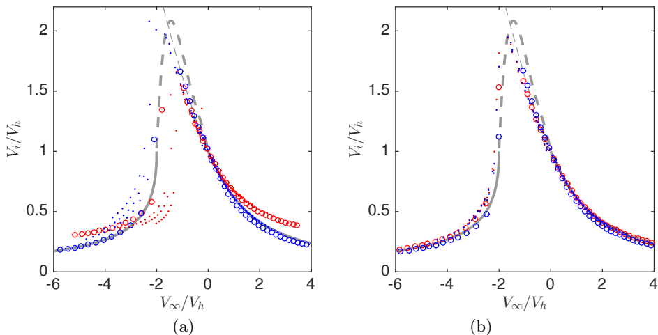
FIGURE 16. Mean induced velocity V_i/V_h versus V_\infty/V_h where V_h is the mean induced velocity in hover for a fixed C_T^{(Hel)} ( C_T^{(Hel)} = 0.01 with circles, C_T^{(Hel)} = 0.02, 0.03, 0.04 with dots). The fixed parameters are N = 2 , \varepsilon = 0.01 . The other parameters are such that -0.2 < 1/\lambda < 0.3 and 0.01 < \eta < 0.1 . The mean induced axial velocity V_i is obtained from V_i = P/T - V_\infty (red symbols) or by taking the mean of U_z^{\text{ind}} in the rotor plane (blue symbols). The solid line is the momentum theory prediction (valid for V_\infty/V_h smaller than -2 or larger than 0 ). The thick dashed line is a fit of experimental data provided by Leishman (2006), eq. (2.96), p. 87. (a) The data are computed using formula (3.5a) for T and (3.6) for P . (b) The data are computed neglecting U_\theta^{\text{ind}} in (3.5a) for T and using \langle U_z^{\text{ind}} \rangle_\theta instead of U_z^{\text{ind}} in (3.6) for P .
