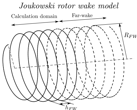
FIGURE 3. Schematic of the complete vortical structure generated at the wake (to simplify the figure, only the tip vortex from a single blade is represented). In solid line, the calculation domain. In dashed line, the prescribed far-wake structure. A smaller number of turns are shown compared to what is used for the computation.
