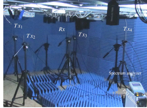
Figure 7: Measurement setup deployed in an quasi-anechoic chamber
