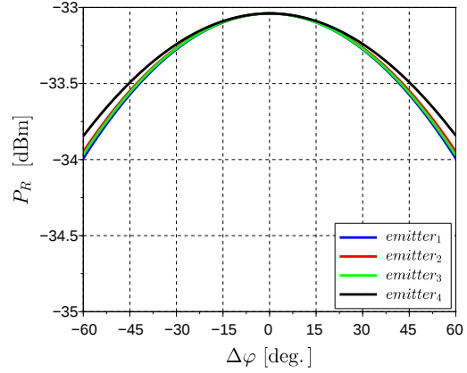
Figure 4: The received power level variation with respect to the deviation of the desired phases \phi_i
