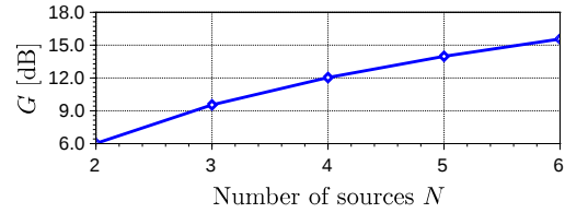
Figure 2: The gain in terms of received power
