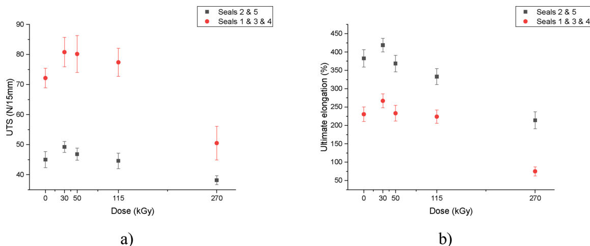
Fig. 7. Ultimate tensile strength (UTS) for seals 2 and 5 (black squares) and seals 1, 3 and 4 (red spheres) – left and Ultimate elongation for seals 2 and 5 (black squares) and seals 1, 3 and 4 (red spheres) – right. The average of all the bag lots is represented for each gamma irradiation dose.
