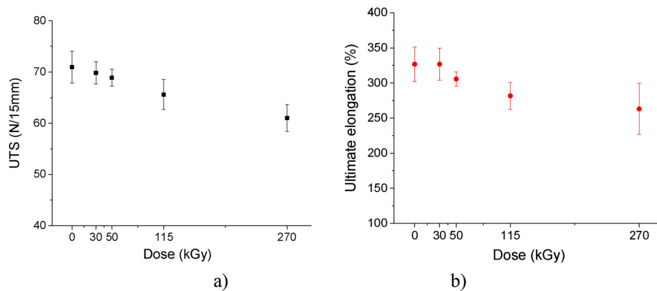
Fig. 10. Ultimate tensile strength (UTS)- a) and ultimate elongation – b). The average of all bag lots is represented for each gamma irradiation dose.
