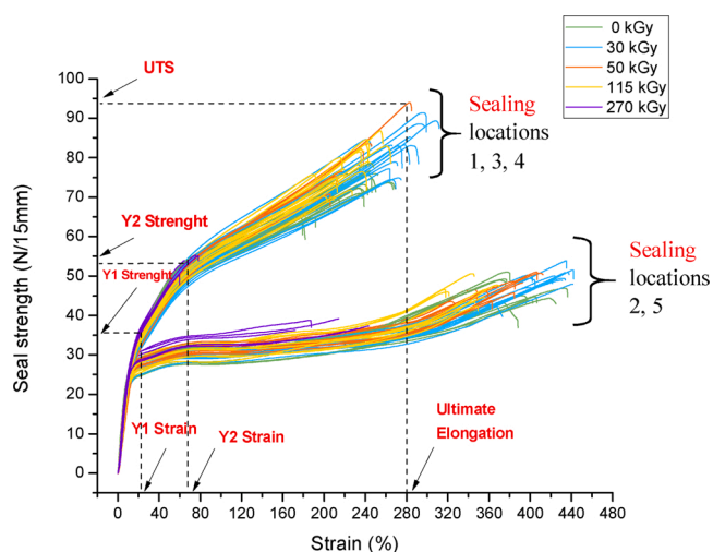
Fig. 4. Strength-strain curves for each seal location (1-5) and each gamma dose (0-270 kGy) for the EVA bags. Colors according to gamma doses.
