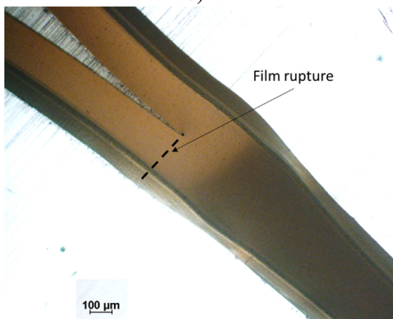
Fig. 3. Example of one of EVA seals before the beginning of the tensile test (a) seal after the end of the tensile test. The seal was not impacted by the test (no opening, no break), only the film was broken (b). Optical microscope pictures of the EVA bag seal (c) and PE bag seal (d).
