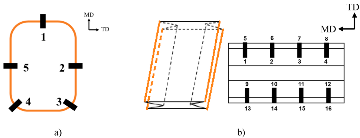
Fig. 2. Five seal locations on EVA bags (a) and 16 seal locations on PE bags (b). Black dashes correspond to seal samples (1-5 for (a) and 1-16 for (b)). Orange lines show where sealing is performed.
