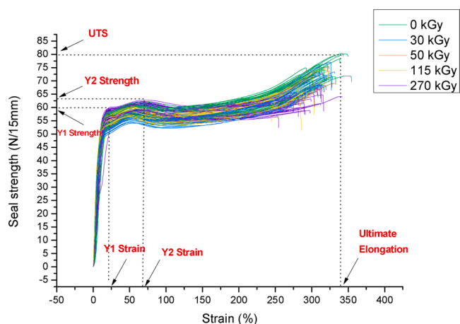
Fig. 8. Strength-strain curves for each seal location (1-16) and each gamma irradiation dose (0-270 kGy) for the PE bags. Colors according to gamma doses.
