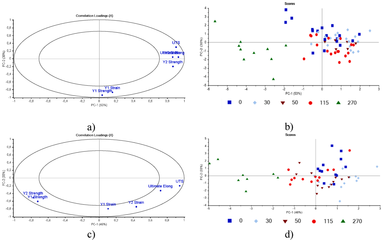
Fig. 6. PCA performed on the six characteristic points of each tensile curve for the EVA bags obtained for 2 lots, all gamma doses. a) Correlation loadings for seals 1,3 and 4. b) Score plots with gamma doses for seals 1, 3 and 4. c) Correlation loadings for seals 2 and 5. b) Score plots with gamma doses for seals 2 and 5.
