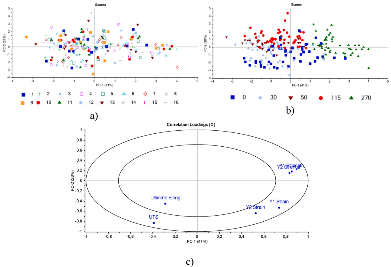
Fig. 9. PCA performed on the six characteristic points of each tensile curve for the PE bags obtained for 2 lots and all gamma doses. a) Score plots with seal locations. b) Score plots with gamma doses. c) Correlation loadings (ellipses represent 75 % and 100 % of the correlation).
