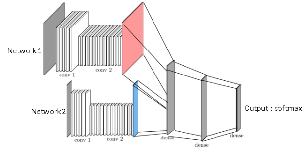
Figure 1: Network architecture
