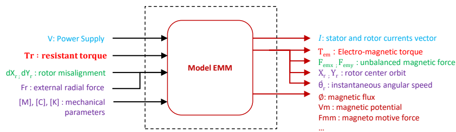
FIGURE 3 – Electro-magneto-mechanical model
