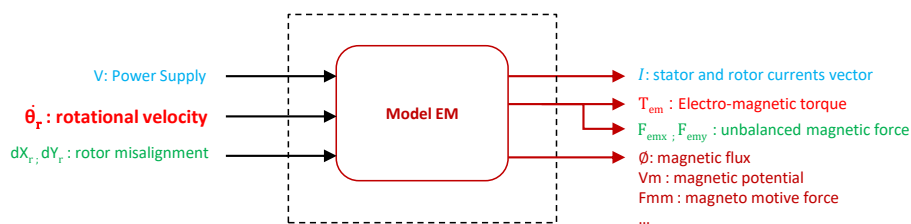
FIGURE 2 – Electro-Magnetic model
