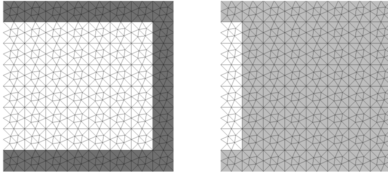
Figure 4: First geometry. Left: \varpi (highlighted in dark grey). Right: B (highlighted in light grey).
