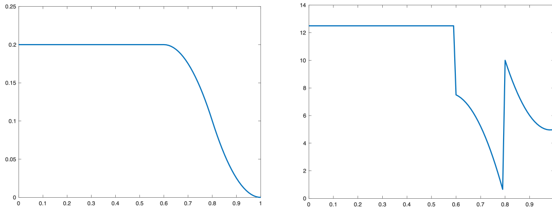
Figure 2: Example of radial cross section of -\tilde{\varphi} (left) and -\mathcal{H}_r(\tilde{\varphi}) (right). The parameter values are r_3 = 1.0 , \zeta = 3 , \delta r = 0.2 , \omega = \delta r \sqrt{2} \sqrt{(2 + \zeta)/(1 + \zeta)} , \kappa = 5 .
