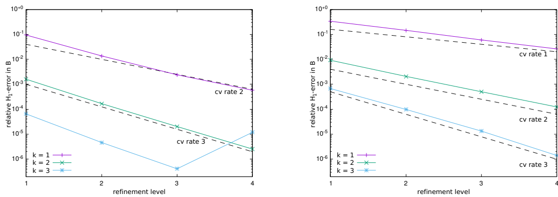
Figure 10: HHO- H^1 -error in B for the first geometry and \omega = 10 . Left: LS-stab. Right: full stab.
