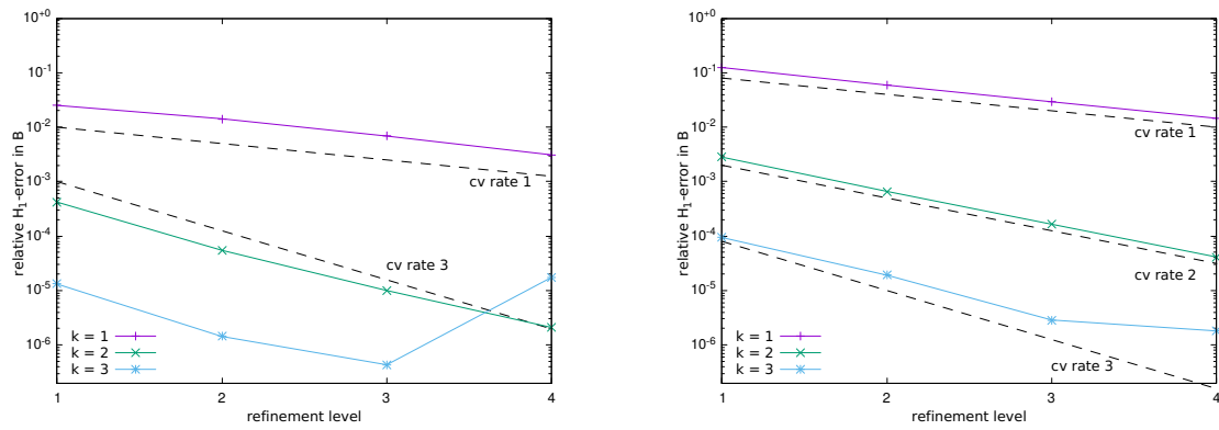
Figure 9: HHO- H^1 -error in B for the first geometry and \omega = 1 . Left: LS-stab. Right: full stab.
