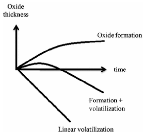
Fig. 2 Schematization of the parabolic behaviour model [7]
