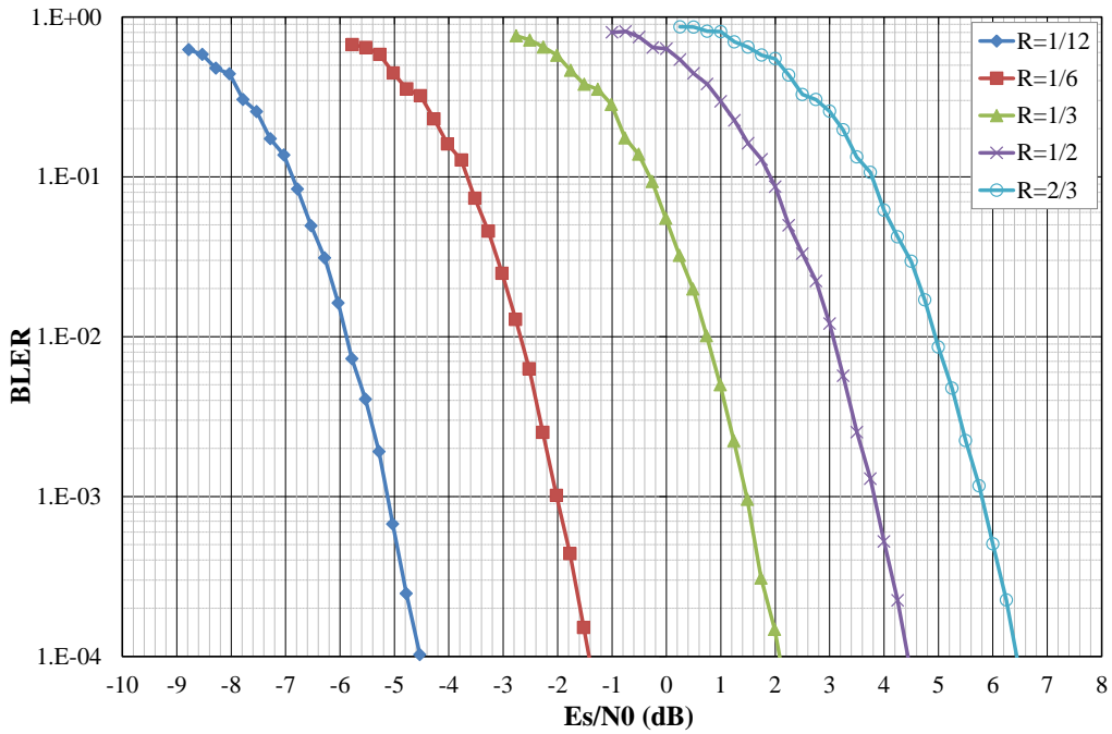
Figure 3: Performance evaluation of the enhanced turbo code in AWGN channel in terms of Block Error Rate vs E_s/N_0 . QPSK modulation , information block size K = 40 bits, 8 decoding iterations of the Max-log-MAP algorithm, tail-biting termination.
