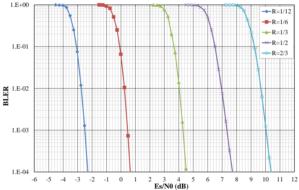
Figure 13: Performance evaluation of the enhanced turbo code in AWGN channel in terms of Block Error Rate vs E_s/N_0 . 16QAM modulation , information block size K = 600 bits, 8 decoding iterations of the Max-log-MAP algorithm, tail-biting termination.
