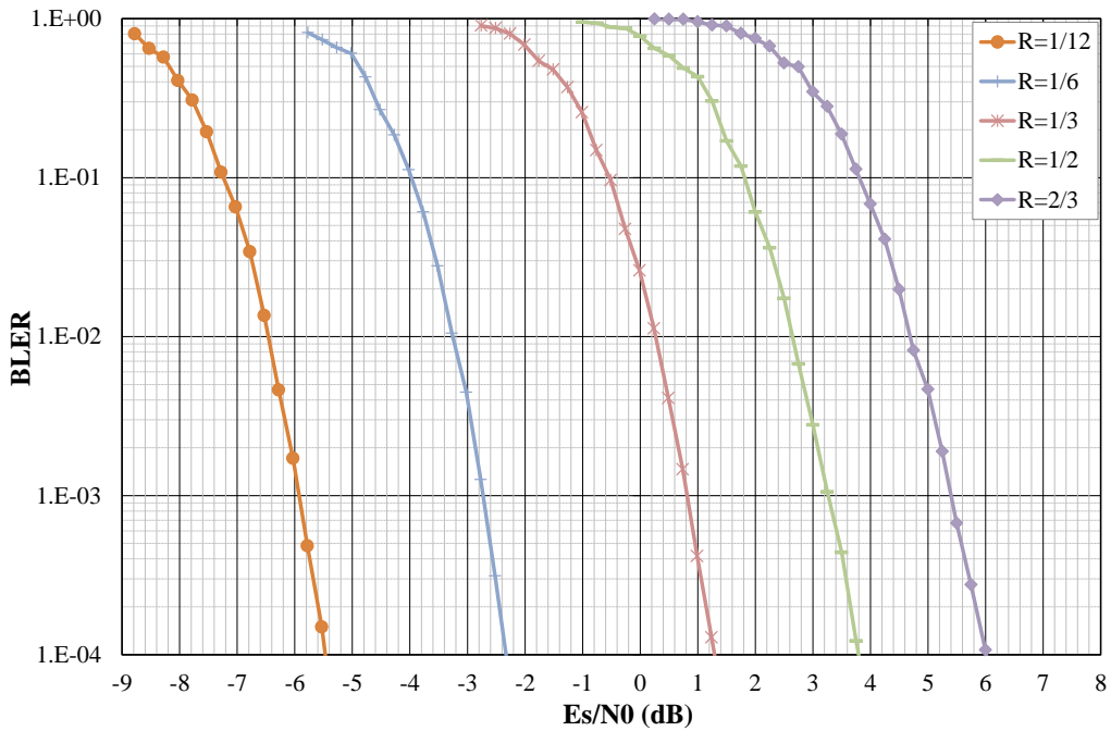
Figure 5: Performance evaluation of the enhanced turbo code in AWGN channel in terms of Block Error Rate vs Es/N0. QPSK modulation , information block size K = 80 bits, 8 decoding iterations of the Max-log-MAP algorithm, tail-biting termination.
