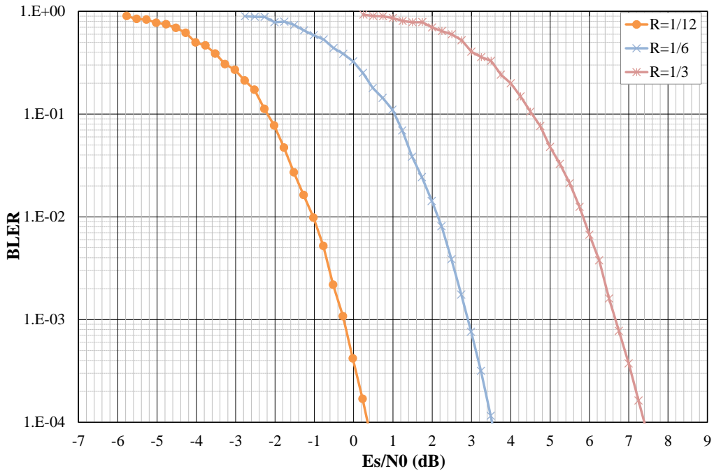
Figure 9: Performance evaluation of the enhanced turbo code in AWGN channel in terms of Block Error Rate vs E_s/N_0 . 16QAM modulation , information block size K = 32 bits, 8 decoding iterations of the Max-log-MAP algorithm, tail-biting termination.
