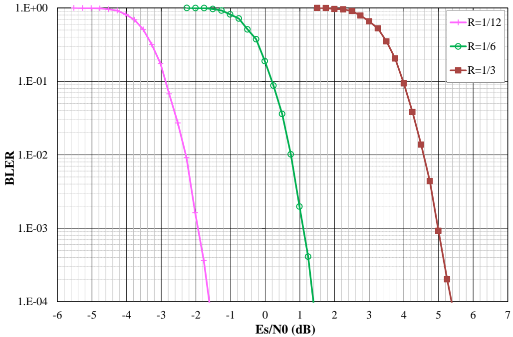
Figure 11: Performance evaluation of the enhanced turbo code in AWGN channel in terms of Block Error Rate vs E_s/N_0 . 16QAM modulation , information block size K = 208 bits, 8 decoding iterations of the Max-log-MAP algorithm, tail-biting termination.
