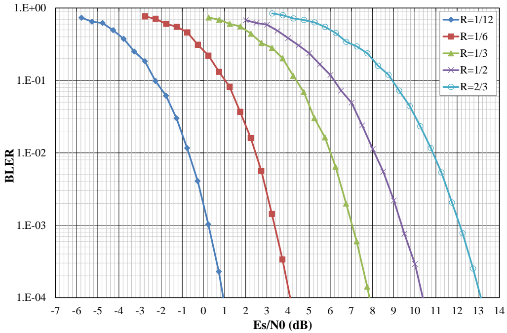
Figure 8: Performance evaluation of the enhanced turbo code in AWGN channel in terms of Block Error Rate vs E_s/N_0 . 16QAM modulation , information block size K = 20 bits, 8 decoding iterations of the Max-log-MAP algorithm, tail-biting termination.
