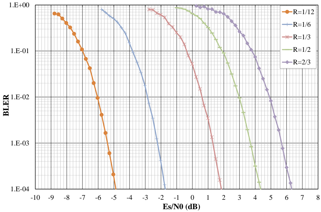
Figure 4: Performance evaluation of the enhanced turbo code in AWGN channel in terms of Block Error Rate vs Es/N0. QPSK modulation , information block size K = 48 bits, 8 decoding iterations of the Max-log-MAP algorithm, tail-biting termination.
