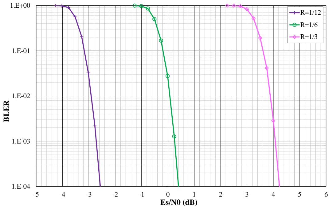
Figure 14: Performance evaluation of the enhanced turbo code in AWGN channel in terms of Block Error Rate vs E_s/N_0 . 16QAM modulation , information block size K = 992 bits, 8 decoding iterations of the Max-log-MAP algorithm, tail-biting termination.
