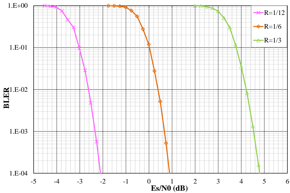
Figure 12: Performance evaluation of the enhanced turbo code in AWGN channel in terms of Block Error Rate vs E_s/N_0 . 16QAM modulation , information block size K = 400 bits, 8 decoding iterations of the Max-log-MAP algorithm, tail-biting termination.
