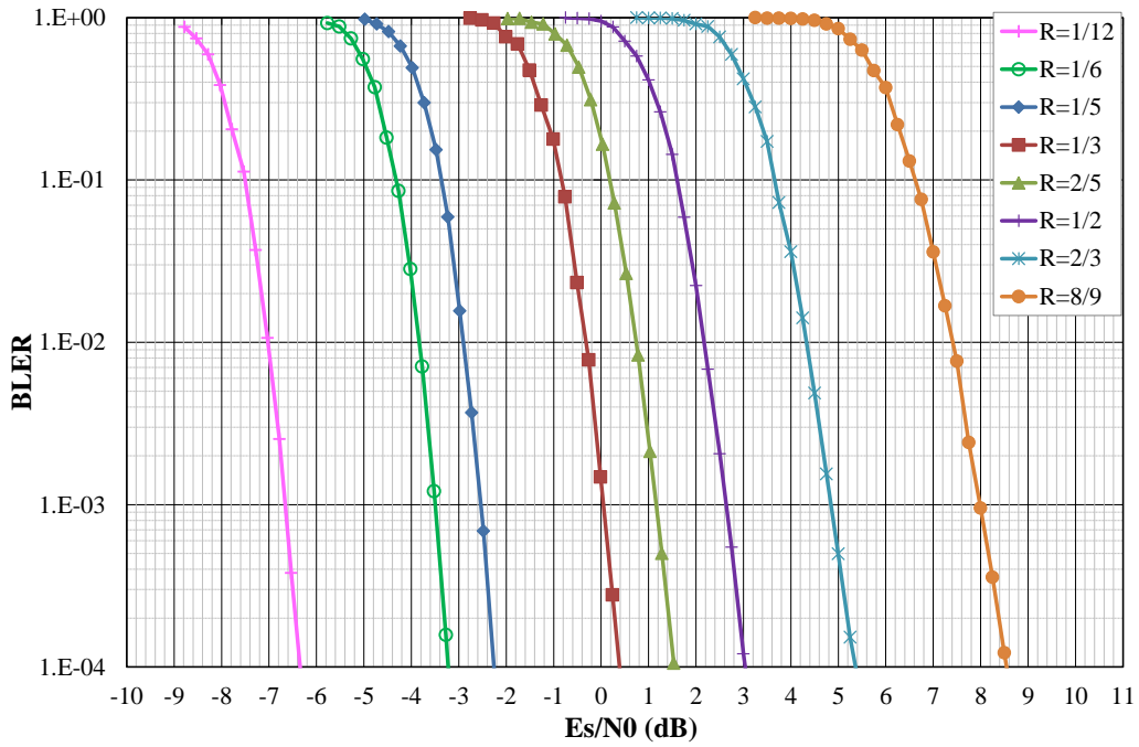
Figure 6: Performance evaluation of the enhanced turbo code in AWGN channel in terms of Block Error Rate vs E_s/N_0 . QPSK modulation , information block size K = 208 bits, 8 decoding iterations of the Max-log-MAP algorithm, tail-biting termination. eMBB and URLLC channel Scenarios.
