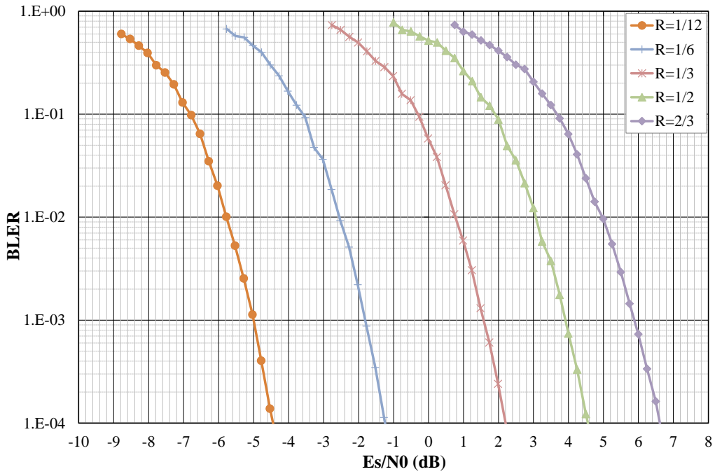
Figure 2: Performance evaluation of the enhanced turbo code in AWGN channel in terms of Block Error Rate vs E_s/N_0 . QPSK modulation , information block size K = 32 bits, 8 decoding iterations of the Max-log-MAP algorithm, tail-biting termination.
