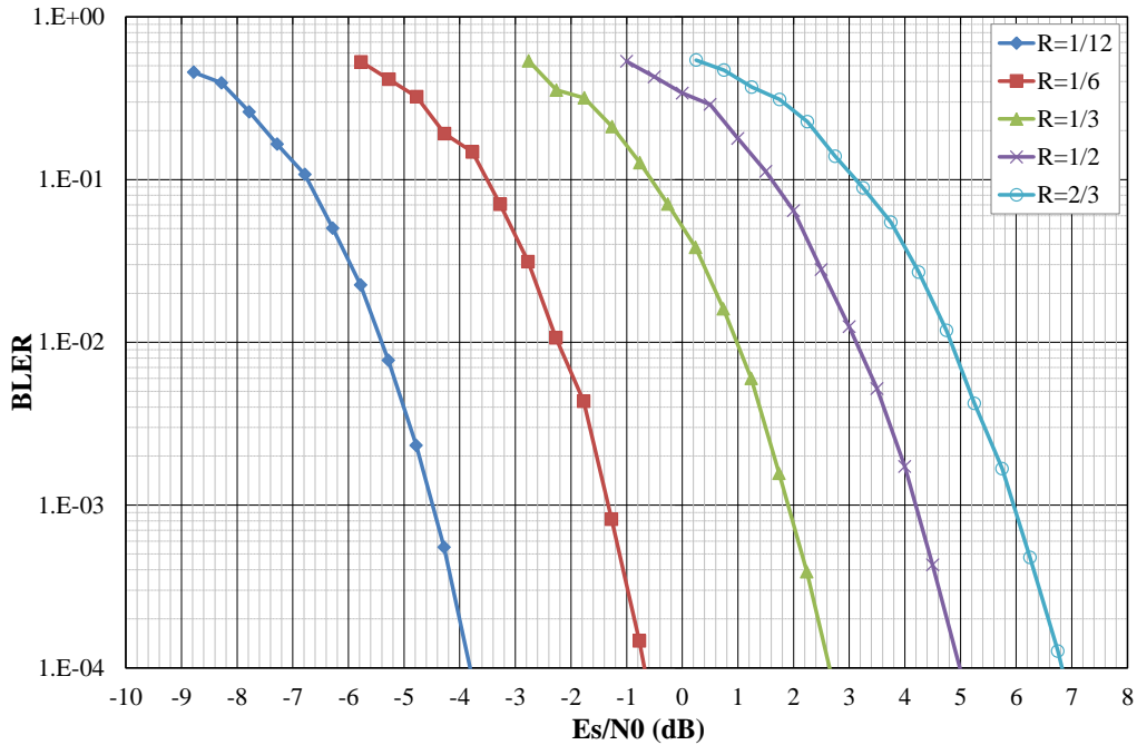
Figure 1: Performance evaluation of the enhanced turbo code in AWGN channel in terms of Block Error Rate vs E_s/N_0 . QPSK modulation , information block size K = 20 bits, 8 decoding iterations of the Max-log-MAP algorithm, tail-biting termination.
