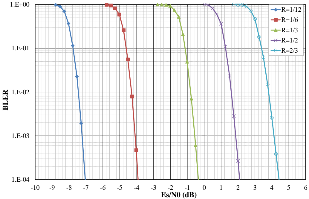
Figure 7: Performance evaluation of the enhanced turbo code in AWGN channel in terms of Block Error Rate vs E_s/N_0 . QPSK modulation , information block size K = 600 bits, 8 decoding iterations of the Max-log-MAP algorithm, tail-biting termination.
