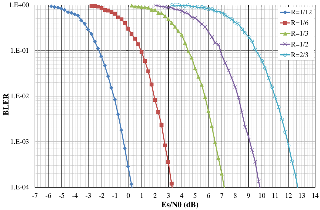
Figure 10: Performance evaluation of the enhanced turbo code in AWGN channel in terms of Block Error Rate vs E_s/N_0 . 16QAM modulation , information block size K = 40 bits, 8 decoding iterations of the Max-log-MAP algorithm, tail-biting termination.
