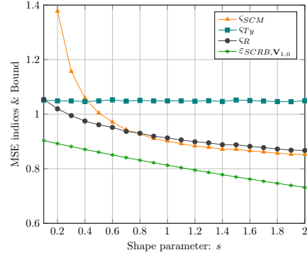
Fig. 2: Estimation of the shape matrix: MSE indices and SCR\mathbf{B} vs s ( L = 5N and 10^6 Monte Carlo runs).
