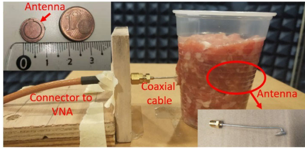
FIGURE 13. Experiment antenna model (porcine meat).
