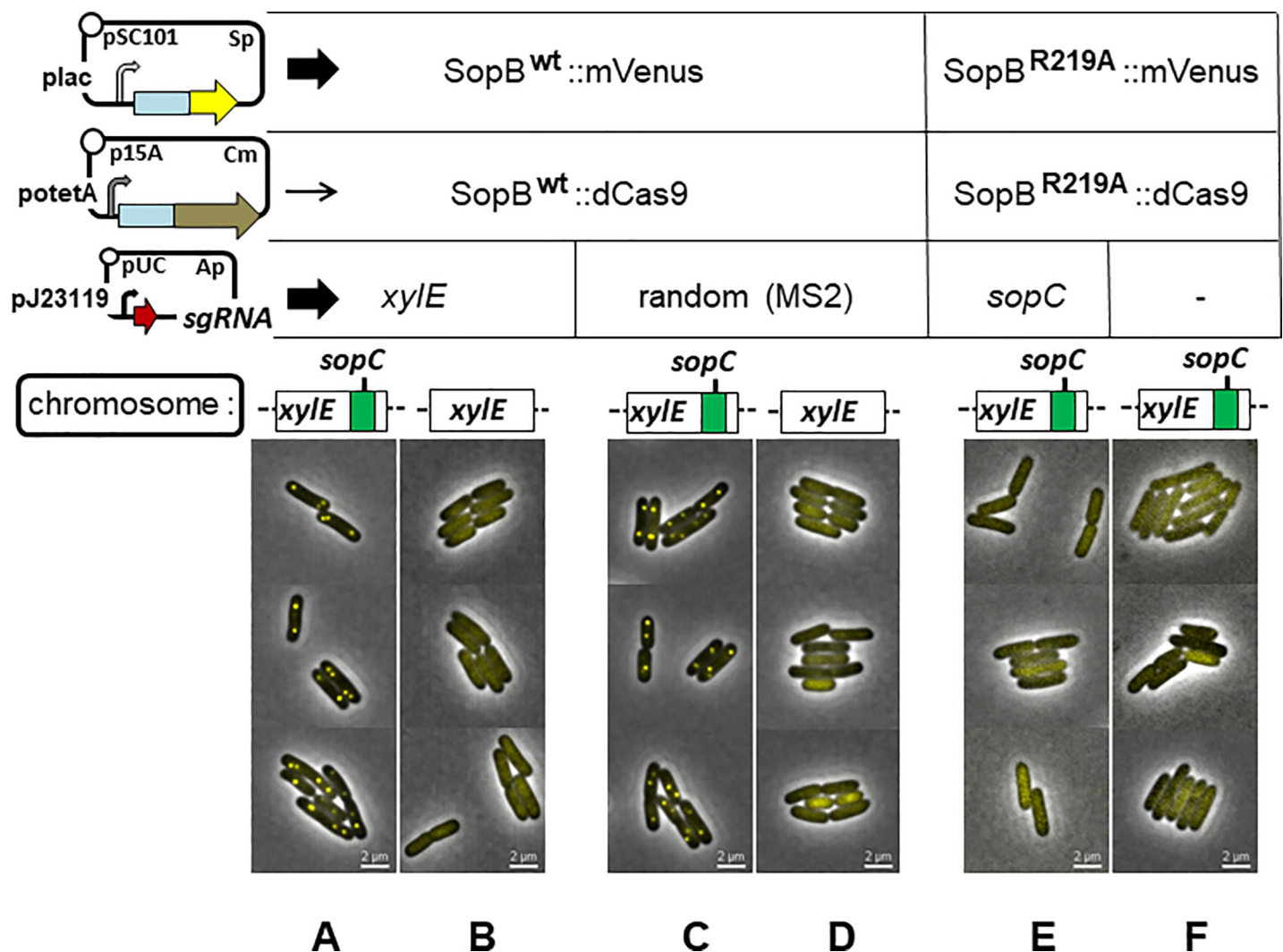
Fig 2. Test of SopB spreading from dCas9-DNA complexes. Cells of strain DLT1215 and its xyleΩsopC derivative, DLT2074, carrying the plasmids that enable SopB visualization and SopB::dCas9 binding (upper left) were applied to buffered agarose-coated slides after at least 10 generations of exponential growth in MGC medium supplemented with and 30μM IPTG; arrow width next to each plasmid indicates the relative level of RNA produced from each. Each column of images shows cells grown with the combination of dCas9 or SopB target sequence, sgRNA, SopB::dCas9 and SopB::mVenus fusion directly above.
