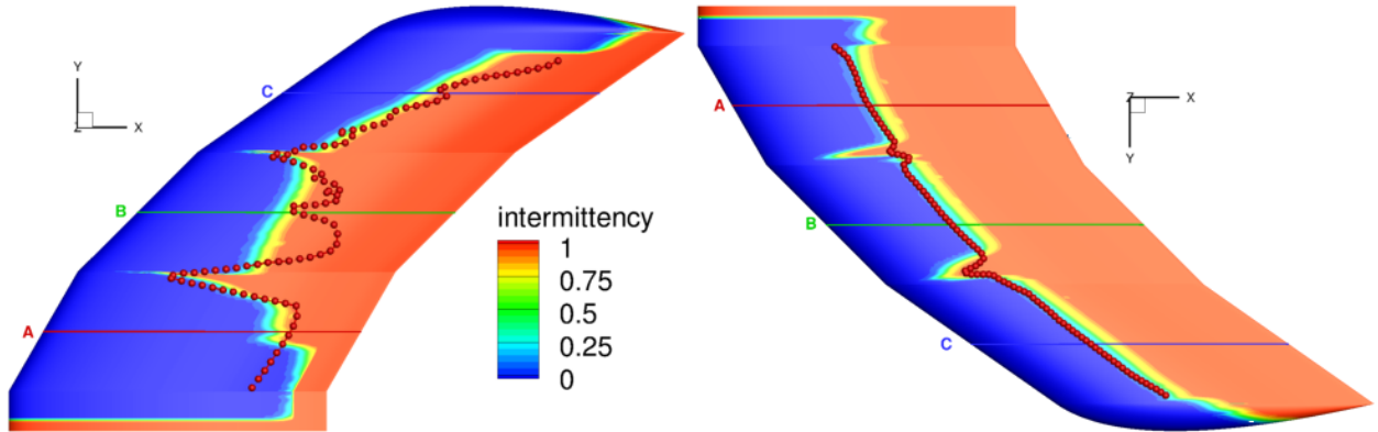
Fig. 5 Sickle wing, case A - Contours of \gamma compared to the experimentally measured transition locations at the suction (left) and pressure (right) sides.
