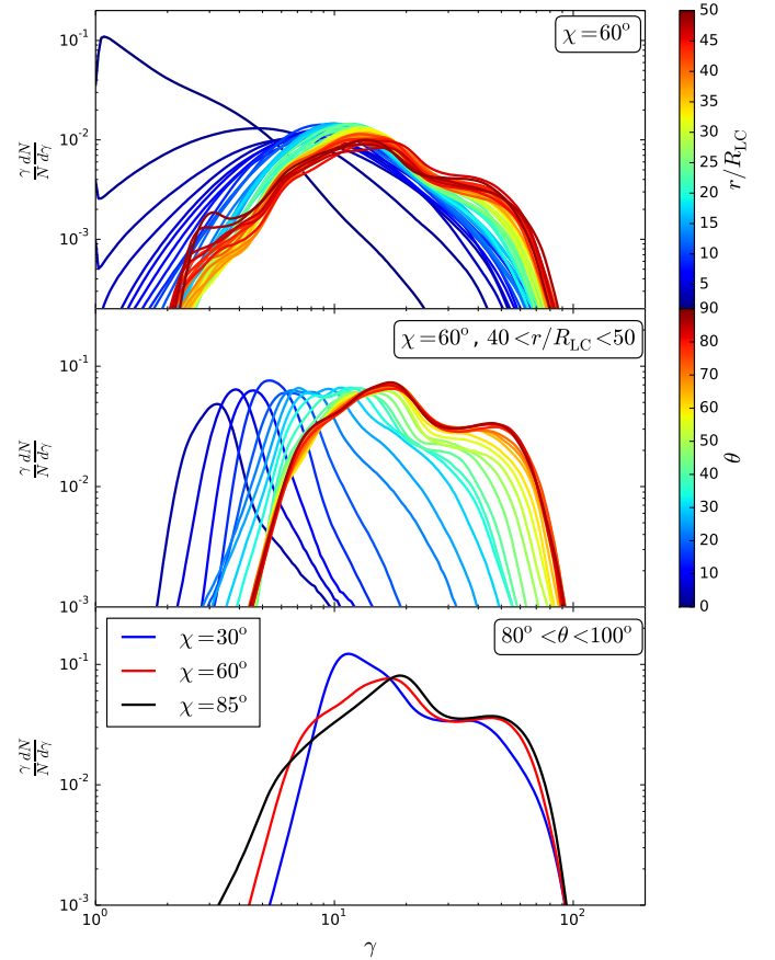
Fig. 7. Top panel: normalized particle energy spectrum, (\gamma/N)dN/d\gamma , within the spherical shells of radius r and r + R_{\text{LC}} as a function of radius (color-coded) for \chi = 60^\circ . Middle panel: latitudinal dependence (color-coded) of the particle energy spectrum averaged between 40 \leq r/R_{\text{LC}} \leq 50 for \chi = 60^\circ . Bottom panel: total particle spectra beyond r = 40 R_{\text{LC}} and 80^\circ \leq \theta \leq 100^\circ for \chi = 30^\circ, 60^\circ , and 85^\circ .
