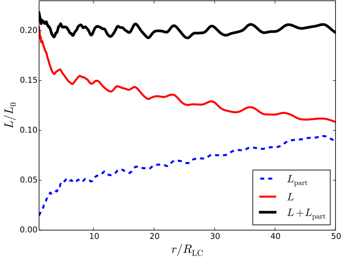
Fig. 4. Radial evolution of the kinetic energy flux carried by the particles, L_{\text{part}} = \iint n(\gamma-1)m_e c^2 v_r r^2 \sin\theta d\theta d\phi (dashed blue line), along with the Poynting flux, L (solid red line) and the total power, L_{\text{tot}} = L + L_{\text{part}} (thick solid black line) for \chi = 60^\circ . Luminosities are normalized by the monopole spindown power L_0 .
