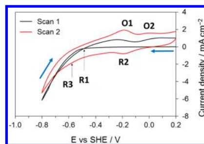
Figure 4. First and second CV scans of the greigite-modified electrode in deoxygenated pH 6.8 0.1 M \text{K}_2\text{HPO}_4/\text{KH}_2\text{PO}_4 solution. Scan rate 0.01 V \text{s}^{-1} . Labels R1–3 and O1–2 are described in the text.
