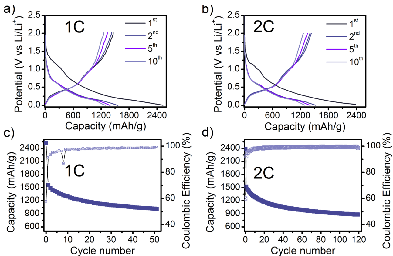
Figure 7. Galvanostatic and their corresponding capacity retention curves for germanane cycled vs Li at the rate of a), c) 1C and b), d) 2C.
