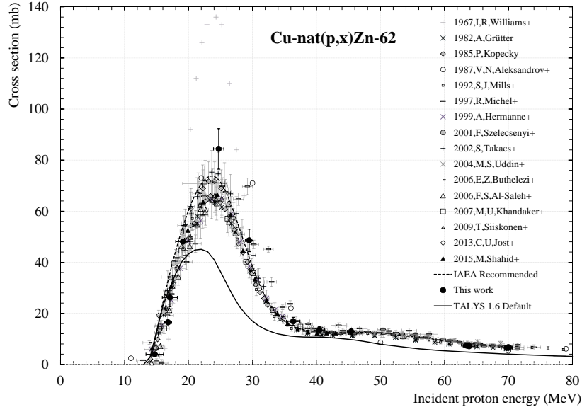
Figure 17: \text{Cu-nat}(p,x)\text{Zn-62} excitation function.
