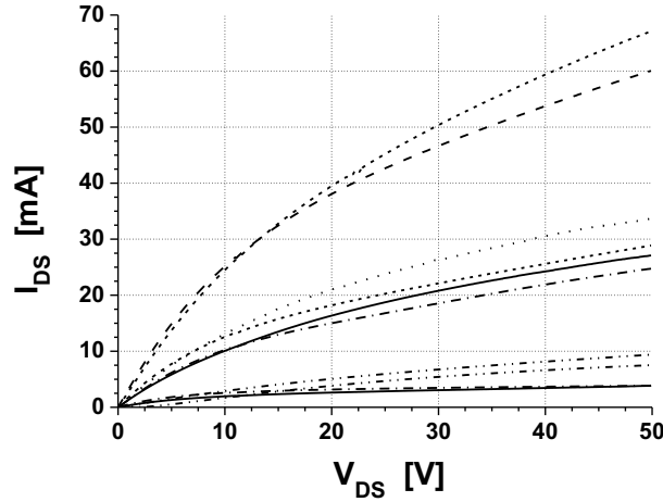
Fig. 3: Sampling of different I-V static characteristics obtained on limiting devices from the first batch (25°C).
