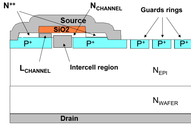
Fig. 1: Vertical cross section of the device and its guard ring peripheral protection (the channel region, L_{\text{CHANNEL}} , and the 'intercell' region are noted).
