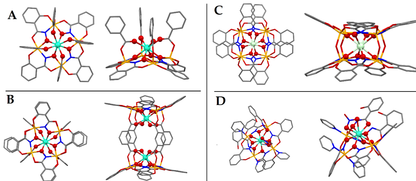
Figure 1. Multiple views of the Ga 3+ /Dy 3+ MCs geometries. (A) [DyGa 4 (shi) 4 (bz) 4 ] corresponding to 1 and 5 . The crystal structure was solved for [DyGa 4 (shi) 4 (bz) 4 (pyH)] ( 1 ), 17 however mass spectrometry and elemental analysis reveal identical molecular composition (Supporting Information). (B) [Dy 2 Ga 8 (shi) 8 (ip) 4 (NH 4 ) 2 ] ( 3 ). 19 (C) [DyGa 8 (shi) 8 (OH) 4 ]Na ( 4 ). 20 The structure was solved for isostructural [NdGa 8 (shi) 8 (OH) 4 ]Na. (D) [DyGa 4 (shi) 4 (H 2 shi) 2 (NO 3 )] ( 2 ). 18 The structure was solved for isostructural [TbGa 4 (shi) 4 (H 2 shi) 2 (NO 3 )], four coordinating pyridines are shown here. Solvents of crystallization, non-integral counter ions, and hydrogen atoms are omitted. Central Ln 3+ and coordinating oxygen atoms are bolded for highlight effect. Color code: Ga-orange; Na-violet; Ln-teal; O-red; N-blue; C-grey.
