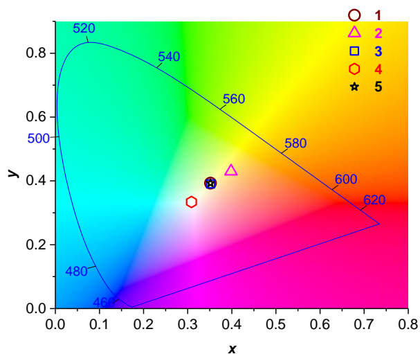
Figure 3. CIE 1931 chromaticity coordinate diagram for 1-5 .
