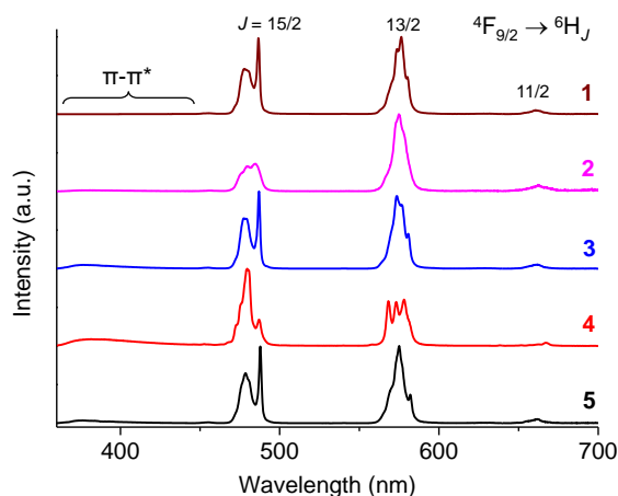
Figure 2. Corrected and normalized emission spectra of Ga 3+ /Dy 3+ MCs in the solid state under excitation at 340 nm, room temp.
