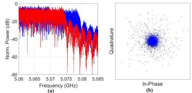
Fig. 3(a) A portion of the transmitted (red) and received (blue) IF signal spectra showing non-overlap due to FO and (b) Constellation of the demodulated signal in an optical heterodyne A-RoF link with free running lasers source and fixed frequency external LO down-conversion receiver.
