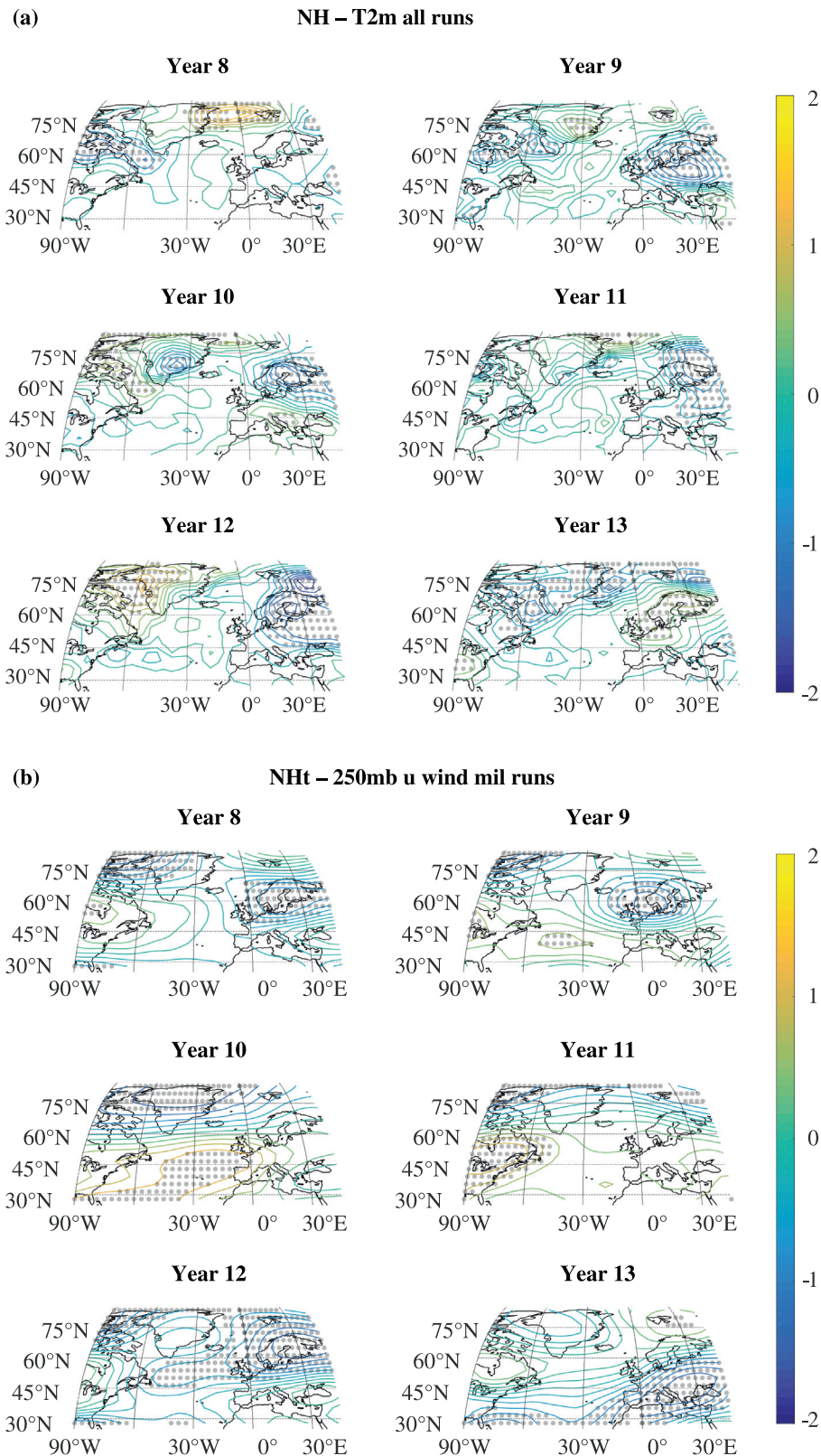
Fig. 7. Composite T2m and u-wind field anomalies 8–13 years after NH eruptions. Anomalies are calculated with respect to 15 years prior to each eruption. Dotted areas are significant in the 95% interval according to a Student's t -test where anomalies are calculated according to 15 years prior to each event.
