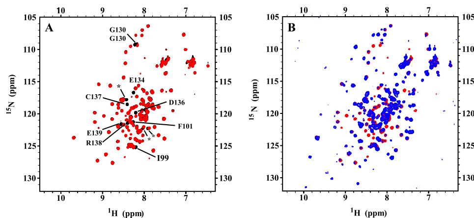
FIGURE 3. Monitoring reduction and zinc titration of Fur monomer by NMR. A , superposition of the ^1\text{H},^{15}\text{N} -HSQC spectra of the oxidized ( black ) and reduced monomer ( red ). The annotated peaks correspond to residues that move after the addition of 1 eq of DTT. B , addition of zinc to DTT-reduced Fur monomer leads to the appearance of the \text{Zn}_5\text{FurD} ^1\text{H},^{15}\text{N} -HSQC spectrum. The correlation peaks of reduced Fur monomer before and after the addition of 0.9 M eq of \text{ZnSO}_4 are shown in red and blue , respectively.
