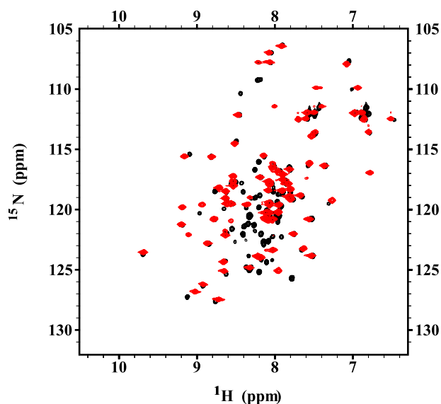
FIGURE 4. Comparison of the ^1\text{H},^{15}\text{N} -HSQC spectra of monomeric Fur and truncated Fur-(1–82). The two spectra are superimposed with the spectrum of monomeric Fur shown in black and that of Fur-(1–82) in red . The black resonance peaks in the center of the spectrum belong to the unstructured C-terminal domain.
