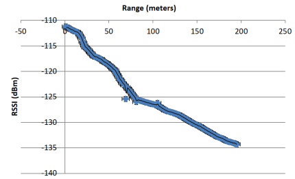
Fig. 1: LoRa range measurement vs. RSSI
