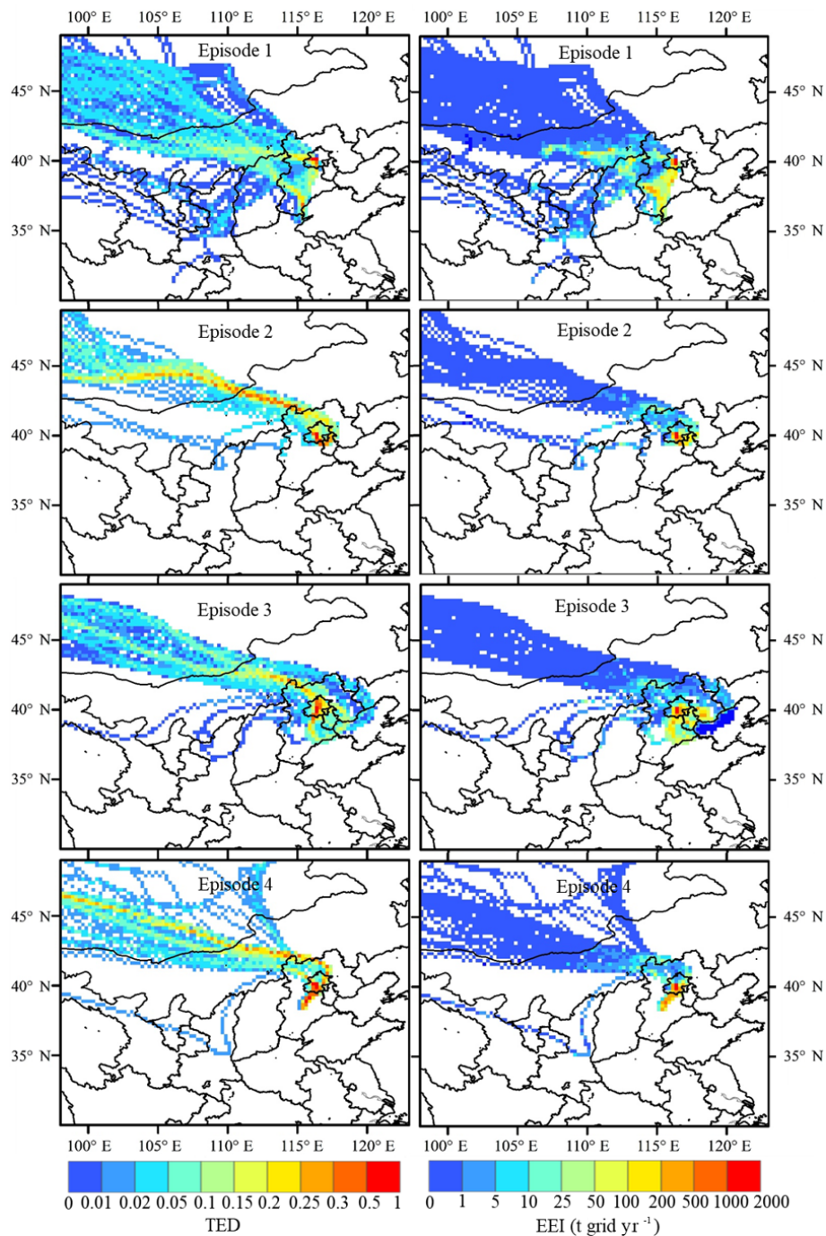
Figure 3. Spatial distribution ( 0.25^\circ \times 0.25^\circ ) of the TED and EEI for BC transported to the observation site ( 40^\circ 00' 17'' N, 116^\circ 19' 34'' E) during episodes 1–4 of the BJNOV2014 measurement period. The TED and EEI were derived from BC emission and black-trajectory analysis (Lu et al., 2012). The TED represents effective trajectory density transported to the receptor site. The EEI quantifies the effective emission amount transported to the receptor site from emission origins.
