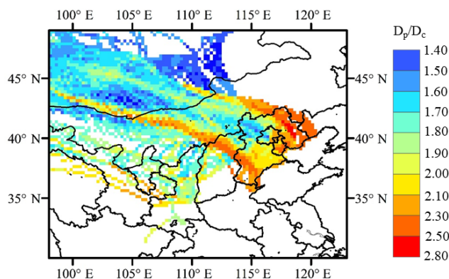
Figure 7. Aging degree (i.e., D_p/D_c ) of BC particles as they are transported to the receptor site ( 40^{\circ}00'17'' N, 116^{\circ}19'34'' E) from emission origins ( 0.25^{\circ} \times 0.25^{\circ} ) during the BJNOV2014 campaign period. The gridded D_p/D_c ratio was calculated by Eq. (11).
