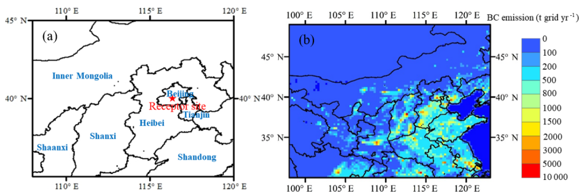
Figure 2. (a) The location of the receptor site (Tsinghua site ( 40^{\circ}00'17'' N, 116^{\circ}19'34'' E), marked as a red star) during the BJNOV2014 measurement period. (b) Spatial distribution ( 0.25^{\circ} \times 0.25^{\circ} ) of the BC emission inventory from MIX.
