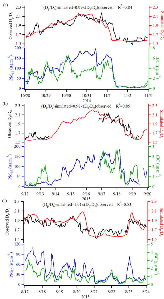
Figure 6. Time series of the observed D_p/D_c ratio, simulated D_p/D_c ratio, and PM_{2.5} and rBC concentrations during the (a) BJNOV2014, (b) BJSEP2015 and (c) BJAUG2015 measurement periods.
