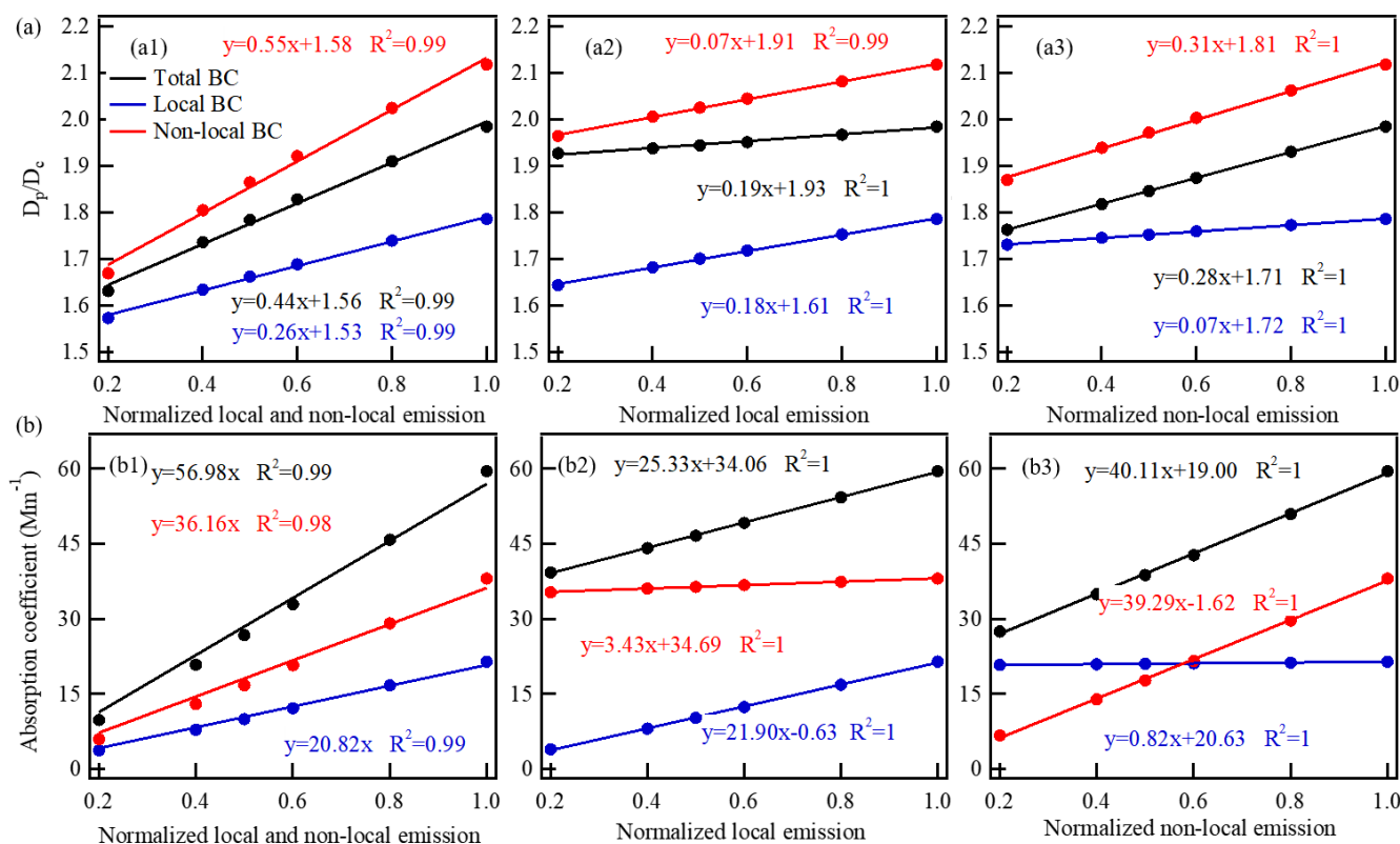
Figure 9. Variations in the (a) D_p/D_c ratio and (b) light absorption coefficient for total, local and non-local BC over the site with normalized emissions. The current emissions obtained from the MIX inventory (Fig. 2b) were normalized as a unit and the emissions reductions of 20 %, 40 %, 50 %, 60 %, and 80 % corresponded to the normalized emissions as 0.8, 0.6, 0.5, 0.4, and 0.2, respectively. (a1) and (b1) represent the simulations for the case of both local and non-local emission variations, respectively; (a2) and (b2) represent the simulations for the case of only local emissions variations; and (a3) and (b3) represent the simulations for the case of only non-local emissions variations. The light absorption coefficient of BC was estimated by the BC mass concentrations, the mass absorption cross section of BC ( 7.5 \text{ m}^2 \text{ g}^{-1} at 550 nm) and the D_p/D_c ratio. When the normalized emissions of total BC were equal to 1, the average mass concentration of total BC was \sim 4.0 \mu\text{g m}^{-3} , which was obtained by measurements during the campaign period. The mass concentration of local and non-local BC can be further calculated based on their EEI contributions (i.e., \sim 1.6 \mu\text{g m}^{-3} for local BC and \sim 2.4 \mu\text{g m}^{-3} for non-local BC). Based on the linear decrease in BC mass concentration with emission reduction, the mass concentrations of total, local and non-local BC for different emission cases were calculated.
