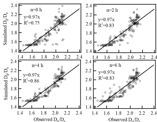
Figure 5. Comparison of the hourly D_p/D_c ratio of BC between the model simulations and observations at our site with different n values in Eq. (13) on 24–30 November 2014 at the Tsinghua site.
