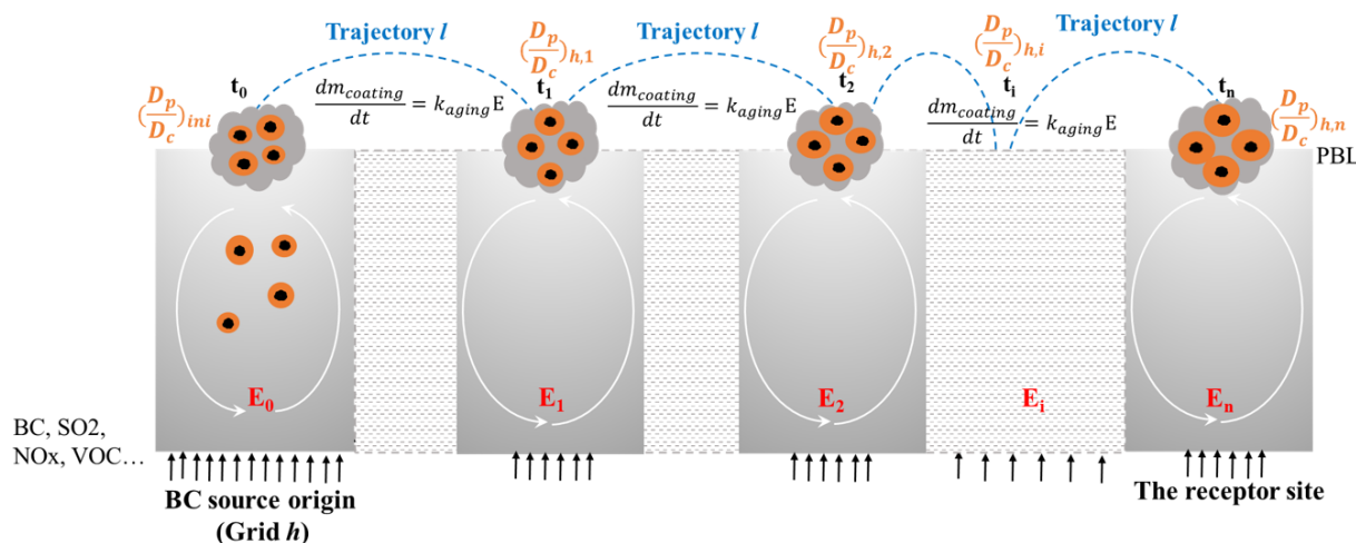
Figure 4. Conceptual scheme of the evolution of the mixing state (i.e., the D_p/D_c ratio) of BC from the source origin (i.e., grid h ) to the receptor site following trajectory l .
