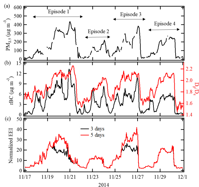
Figure 1. Time series of the PM_{2.5} concentration, rBC mass concentration, D_p/D_c ratio of BC-containing particles and the hourly EEI for BC transported to the observation site for 3-day and 5-day back-trajectories during the BJNOV2014 period.
