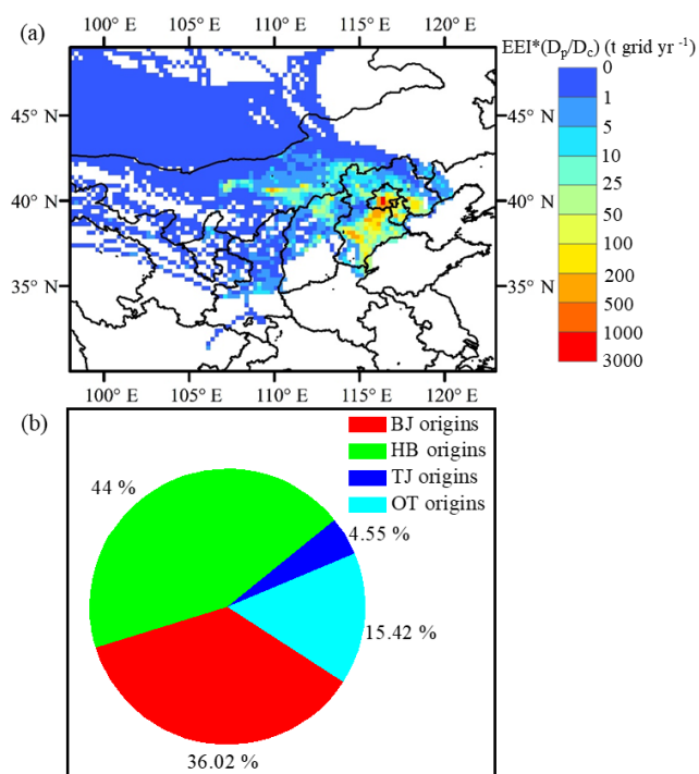
Figure 10. (a) Spatial distribution ( 0.25^\circ \times 0.25^\circ resolution) for light absorption levels (i.e., EEI \times (D_p/D_c) ) of BC as it is transported to the receptor site ( 40^\circ 00' 17'' N, 116^\circ 19' 34'' E) from various source origins. (b) Contributions of different source regions to BC light absorption at the receptor site. The classification of source regions based on political boundaries is shown in Fig. 8a. The BJ, HB, TJ and OT origins represent spatial sources of emitted BC transported to the receptor site from Beijing, Hebei, Tianjin and other regions, respectively.
