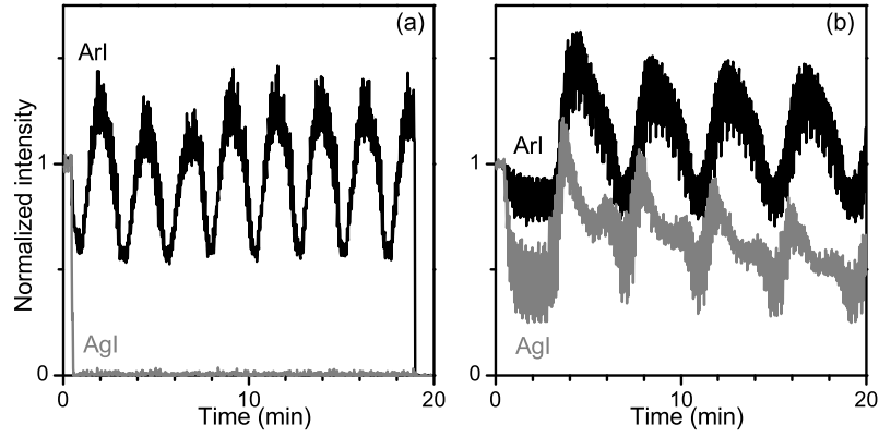
Figure 1. Time-resolved OES of argon (549.6 nm) and silver (546.5 nm) lines. Dust synthesis (a) without silver sputtering ( P=10 W, HMDSO average flow = 0.28 sccm), and (b) with silver sputtering ( P=30 W, HMDSO average flow = 0.12 sccm).
