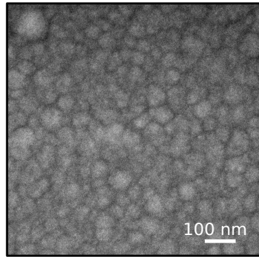
Figure 2. SEM image of collected dust ( P=10 W, HMDSO average flow = 0.28 sccm).
