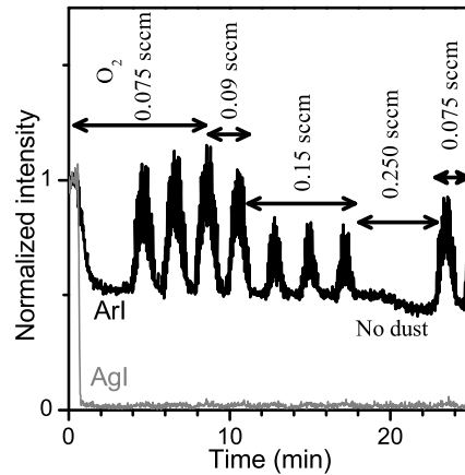
Figure 4. Time resolved OES following the impact of oxygen flow on dust formation.
