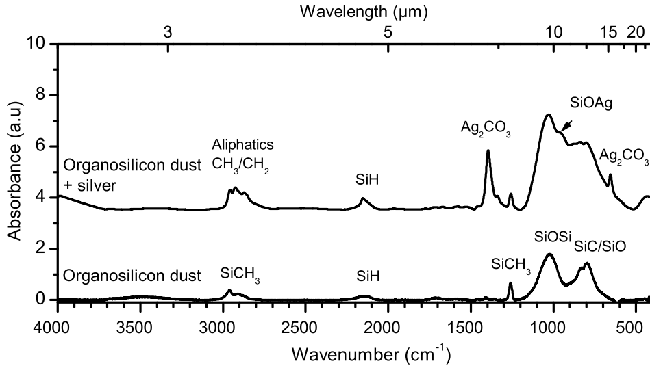
Figure 3. Infrared spectra of collected organosilicon dust with and without silver.
