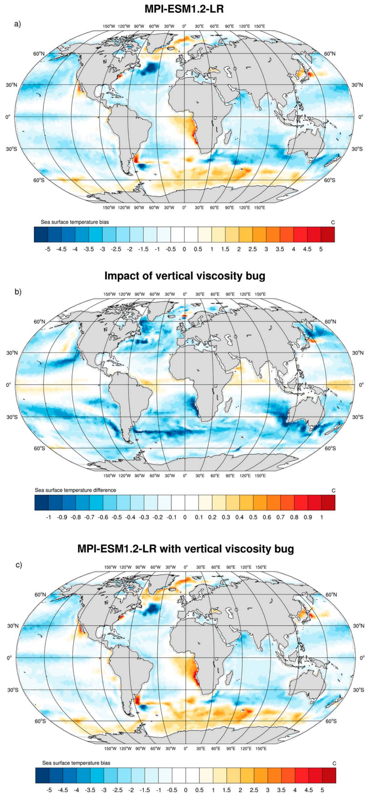
Figure 6. Sea surface temperature biases (50-year average) in preindustrial control simulations with respect to observed climatology (Steele et al., 2001): (a) MPI-ESM1.2-LR after applying the vertical viscosity bug fix and (c) the otherwise identical MPI-ESM1.2-LR but including the coding bug. (b) The difference between (a) and (c); (b) has a different color scale.
