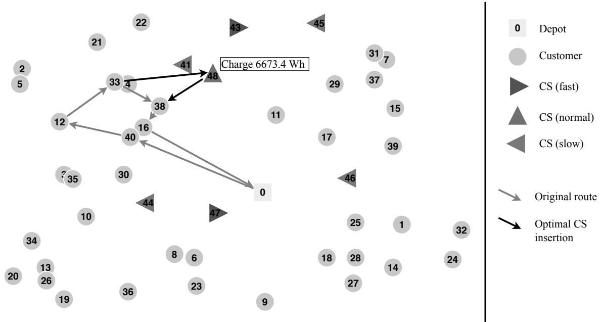
Figure 4: Depiction of example instance “vrprep-instance.xml.” We consider an EV given the route shown by the gray arrows. The solution to the FRVCP for this route instructs the EV to recharge at CS 48 between customers 33 and 38 (black arrows).
