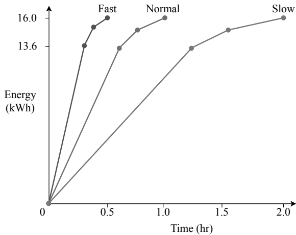
Figure 3: Piecewise linear charging functions for example instance “vrprep-instance.xml.”
