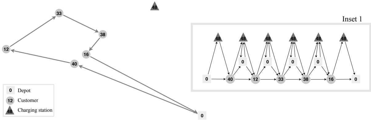
Figure 1: Instance excerpt depicting a fixed route in the original problem graph (left) and the modified problem graph for the FRVCP (Inset 1), which includes dummy nodes for CS insertions.
