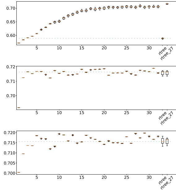
Figure S19: Airbnb dataset. R^2 score of a two-layer tree architecture w.r.t. the second-layer tree depth, when the first-layer (encoding) tree is of depth 10 (top), 27 (middle), and 32 (bottom). rtree is a single tree of respective depth 10 (top), 27 (middle), and 32 (bottom), applied on raw data. For this dataset, the optimal depth of a single tree is 27 and the tree with the optimal depth is depicted as rtree_27 in each plot. The green dashed line indicates the median score of the rtree . All boxplots are obtained by 10 different runs.
