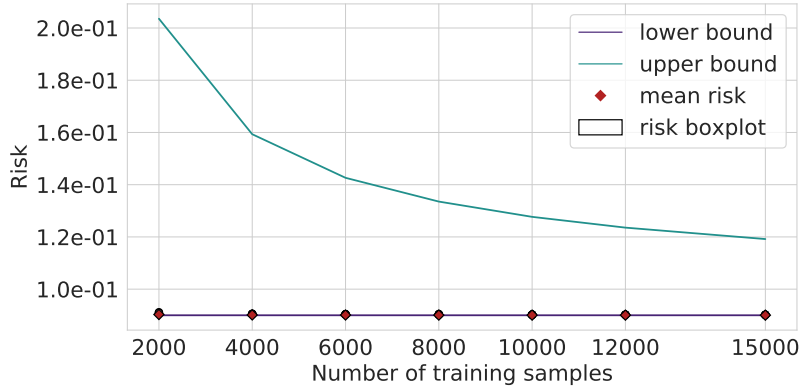
Figure S38: Illustration of the theoretical bounds for a shallow tree network of Proposition 3.2. for a chessboard with parameters k^* = 4 , N_{\mathcal{B}} = 2^{k^*-1} and p = 0.8 . The first-layer tree is of depth k = 2 . We draw a sample of size n (x-axis), and a single tree r_{k,0,n} is fitted for which the theoretical risk is evaluated. Each boxplot is built out of 20 000 repetitions. The outliers are not shown for the sake of presentation. Note that in such a case, the theoretical lower bound is constant and equal to the bias term.
