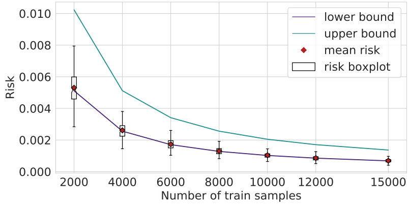
Figure S37: Illustration of the theoretical bounds for a single tree of Proposition 4.1. for a chessboard with parameters k^* = 4 , N_{\mathcal{B}} = 2^{k^*-1} and p = 0.8 . The single tree is of depth k = 6 . We draw a sample of size n (x-axis), and a single tree r_{k,0,n} is fitted for which the theoretical risk is evaluated. Each boxplot is built out of 20 000 repetitions. The outliers are not shown for the sake of presentation.
