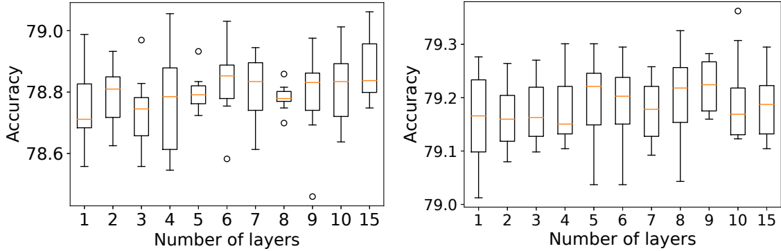
Figure 4: Adult dataset. Boxplots over 10 runs of the accuracy of a DF sub-model with 1 (Breiman) forest by layer (left) or 4 forests (2 Breiman, 2 CRF) by layer (right), depending on the maximal number of layers of the global DF model.
