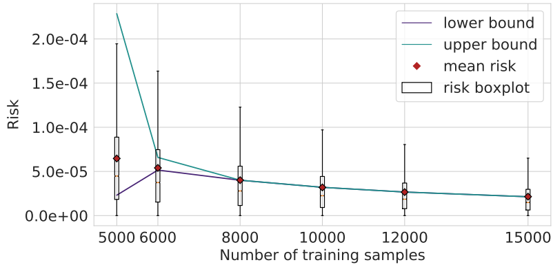
Figure S40: Illustration of the theoretical bounds for a shallow tree network of Proposition 4.2 for a chessboard with parameters k^* = 4 , N_{\mathcal{B}} = 2^{k^* - 1} and p = 0.8 . The first-layer tree is of depth k = 6 . We draw a sample of size n (x-axis), and a single tree r_{k,0,n} is fitted for which the theoretical risk is evaluated. Each boxplot is built out of 20 000 repetitions. The outliers are not shown for the sake of presentation. Note that in such a case, the theoretical lower bound is constant and equal to the bias term.
