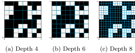
Figure 8: Arbitrary chessboard data distribution for k^* = 6 and N_{\mathcal{B}} = 40 black cells ( p is not displayed here). Partition of the (first) encoding tree of depth 4, 6, 8 (from left to right) is displayed in blue. The optimal depth of a single centered tree for this chessboard distribution is 6.
