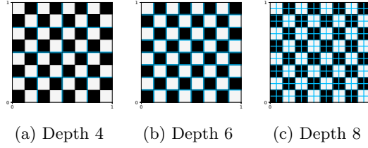
Figure 9: Chessboard data distribution for k^* = 6 and N_{\mathcal{B}} = 2^{k^* - 1} . Partition of the (first) encoding tree of depth 4, 6, 8 (from left to right) is displayed in blue. The optimal depth of a single centered tree for this chessboard distribution is 6.
