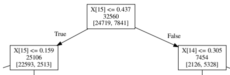
Figure 7: Adult dataset. Focus on the first levels of the second-layer tree structure when the first layer tree is of depth 9 (optimal depth). Raw features range from X[0] to X[13] , X[14] and X[15] are the features built by the first-layer tree.
