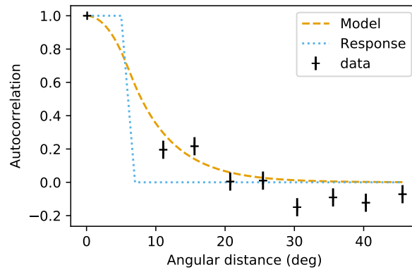
Figure 3: Autocorrelation of the deviations from the best fit empirical disc-like model. The black crosses are the data with errors indicating 1- \sigma confidence intervals. The blue dotted curve is the HaloSat angular response. The yellow dashed curve shows the function w_0(\phi) = e^{-\phi/\phi_a} with \phi_a = 6^\circ convolved with the HaloSat angular response.
