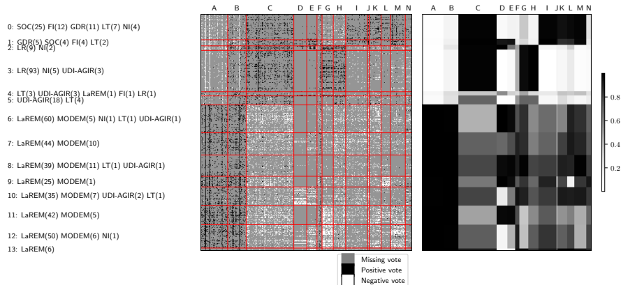
Figure 11: Left: matrix of votes reordered according to the row and column classes, for the MNAR LBM model selected by ICL, with 14 MP classes and 14 text classes. The red lines delineate class boundaries. The counts of MPs belonging to their political groups in each MP class is given on the left. Right: summary of the inferred opinions (expressed or not) for all classes of texts and MPs, as given by the estimated probability to support a text in each block of the reordered matrix.
